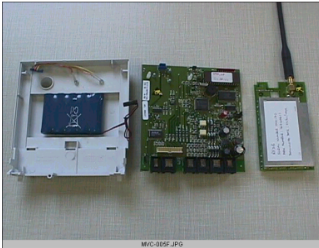
GPT Modem - Case with battery, RF PCB and VIU PCB
