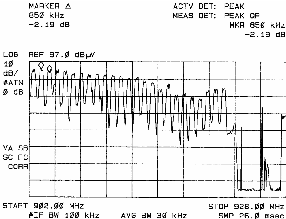
Figure thirteen plot showing at least 25 hopping channels.
