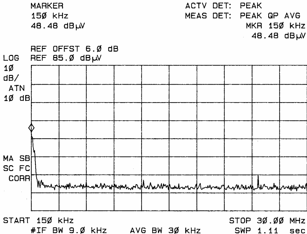
Figure two Conducted Emissions Line 2.
