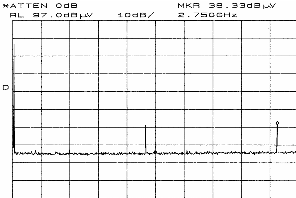
START 900MHZ STOP 2.900GHz *RBW 100KHZ VBW 100KHZ SWP 500ms Figure five Antenna Conducted Emissions taken in the screen room.
