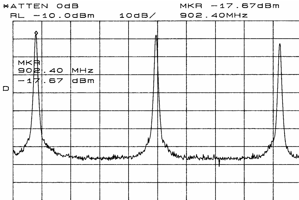
START 900.00MHz STOP 930.00MHz *RBW 100kHz VBW 100kHz SWP 50ms Figure seven Maximum Power outputplot taken in a screen room
