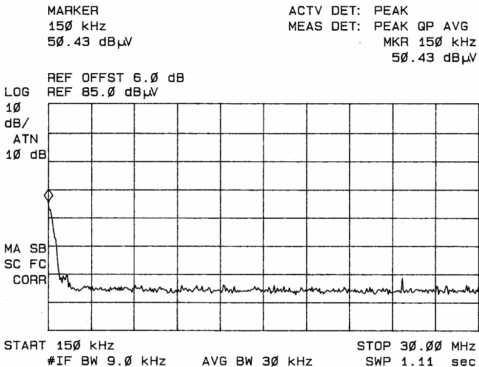
Figure one Conducted Emissions Line 1.
