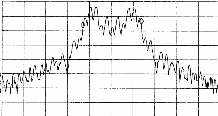
Figure eleven 20-dB bandwidth.
