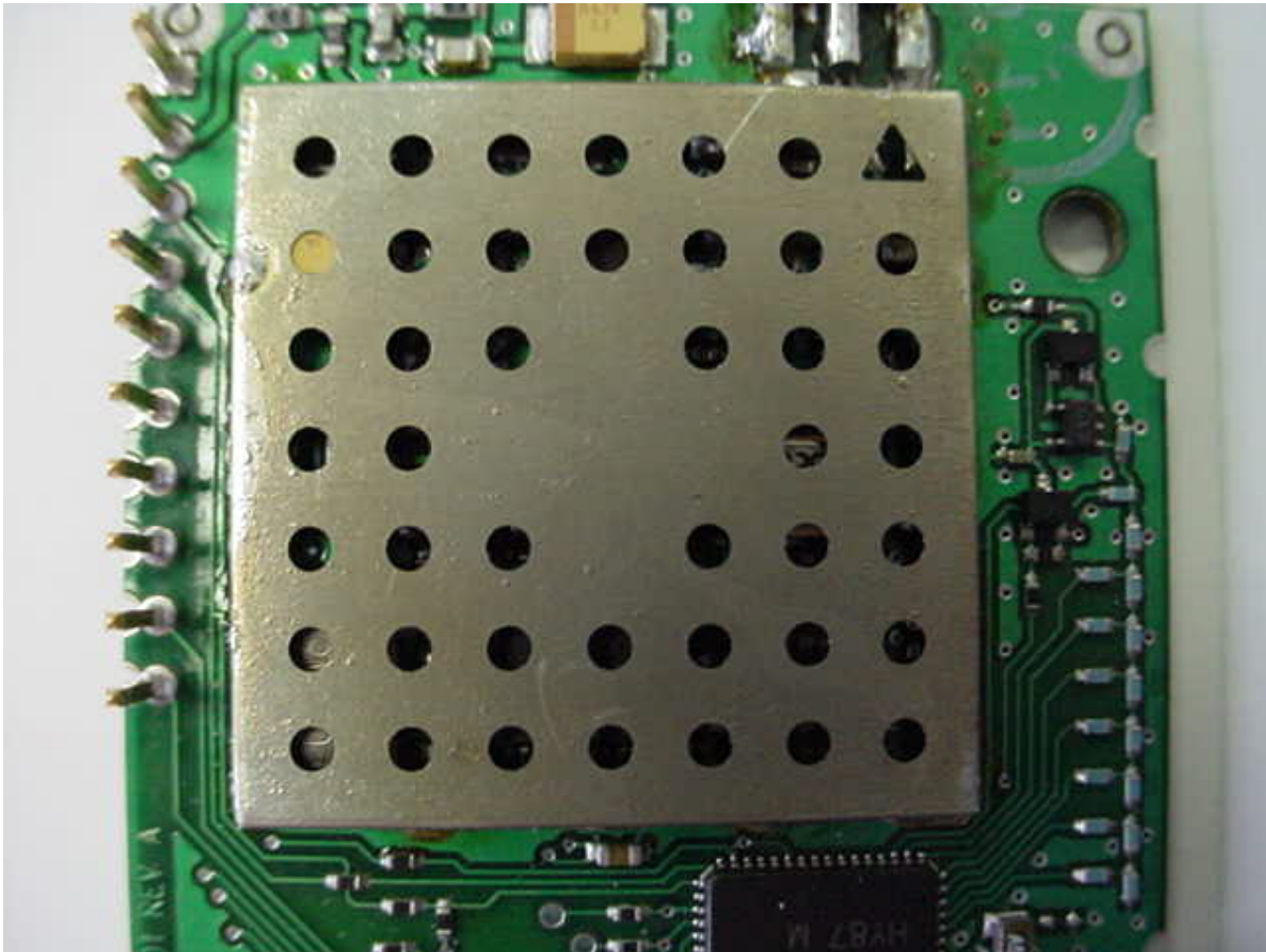
Photo Two – External Close Up of RF Section, Shielded
