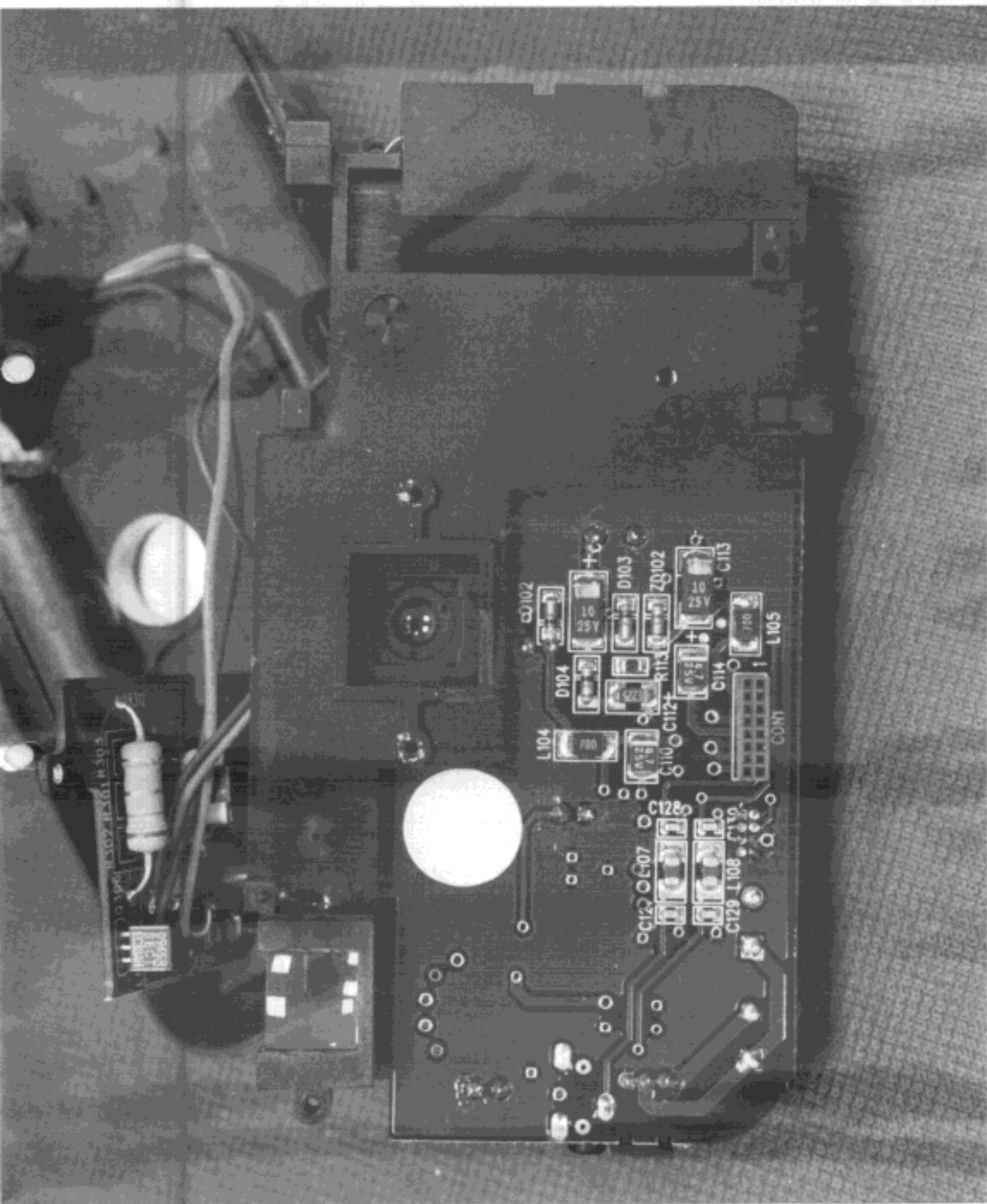
ECC ID: N3DLARGAND601A PHOTO 7. EUT SOLDERING SIDE VIEW
