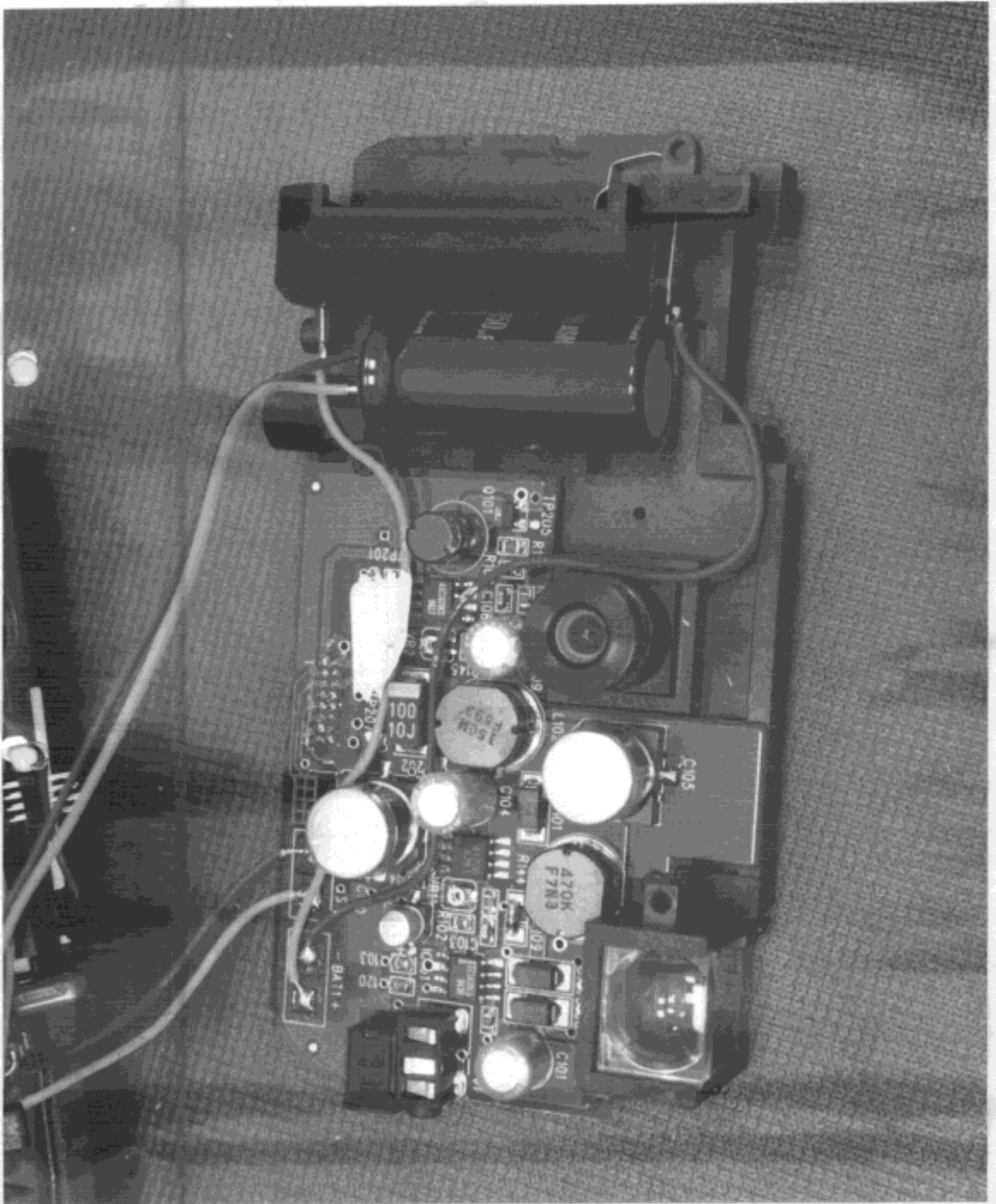
PHOTO 6. EUT COMPONENT SIDE VIEW
