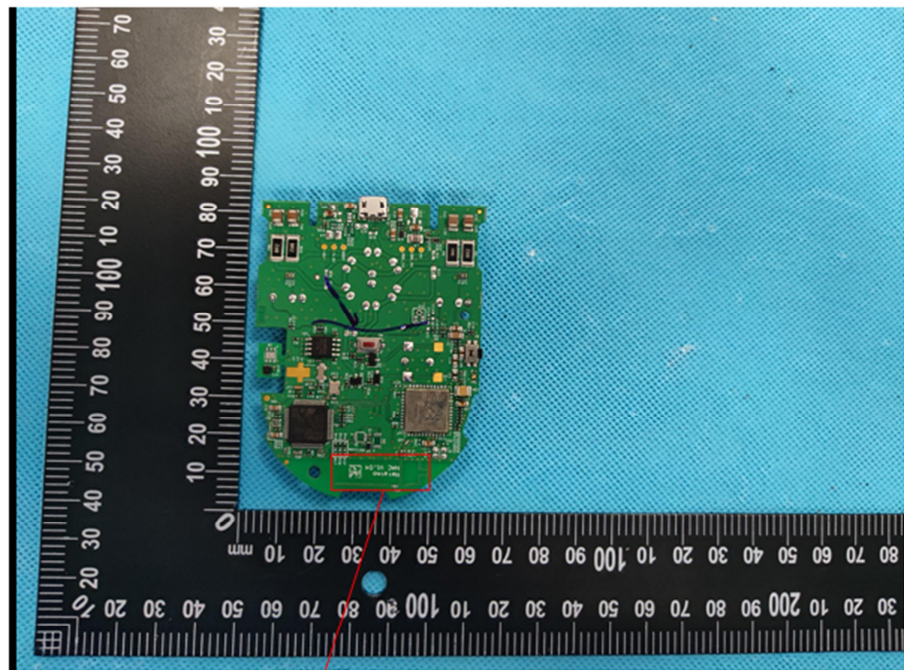
WiFi Antenna
