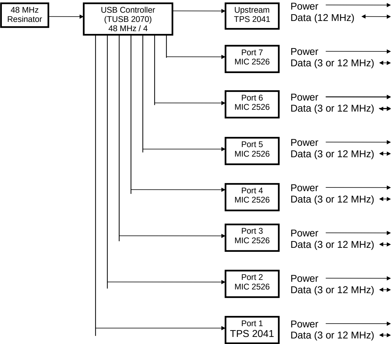
Block Diagram
