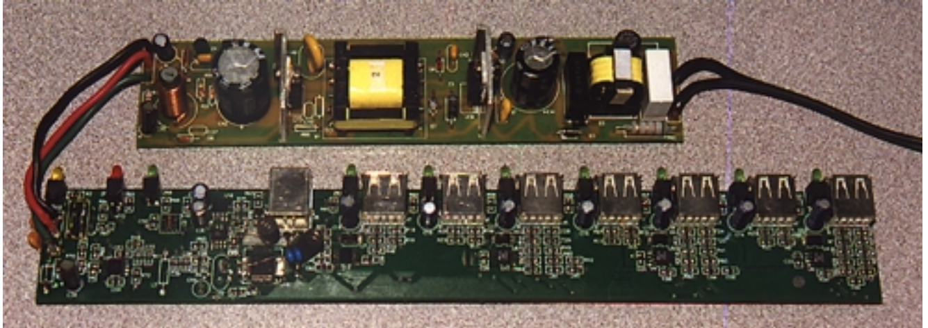
Power Supply - Component Side
