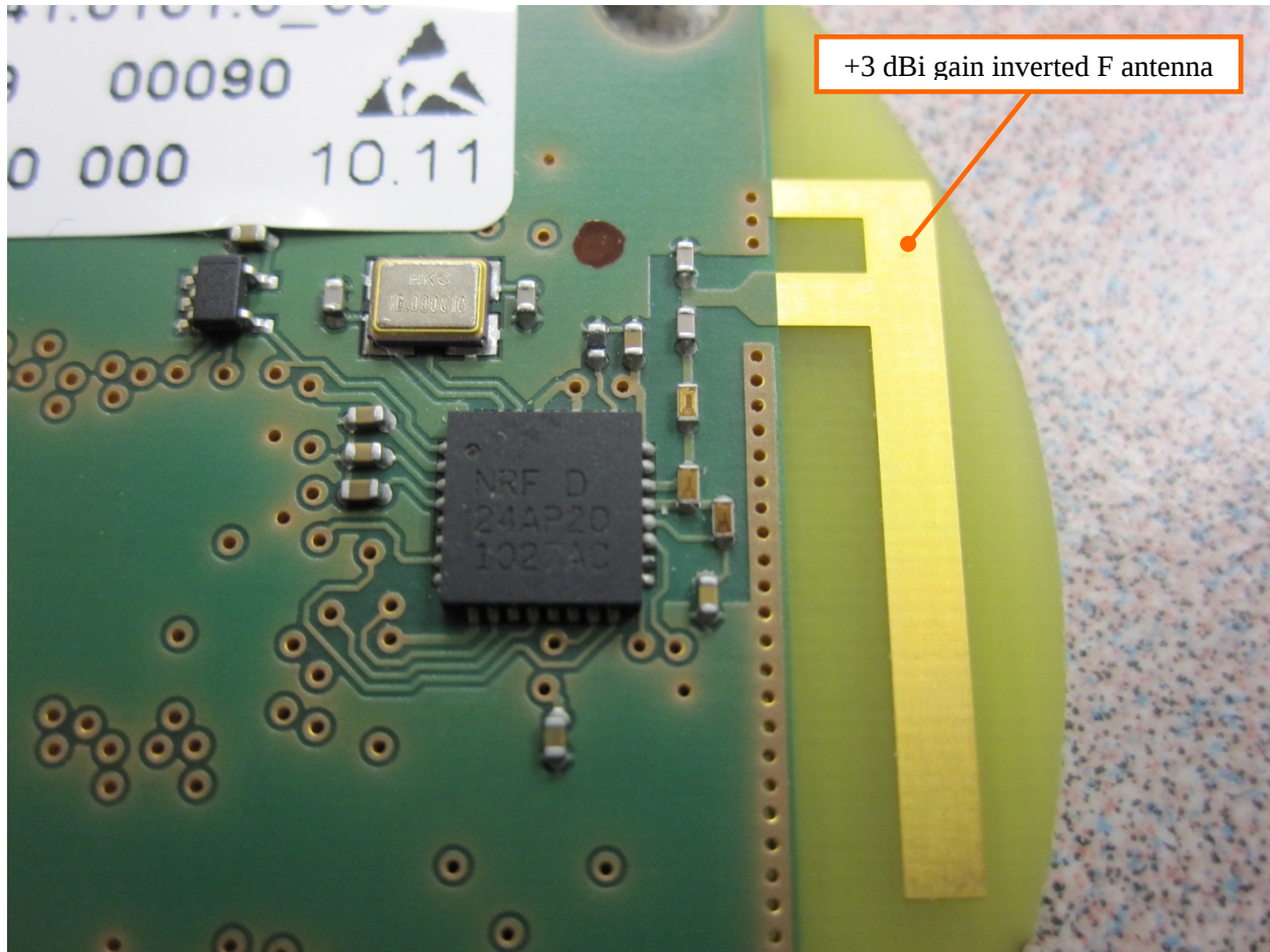
Figure 3: Top close up bottom view of transmitter section of main board and antenna.
