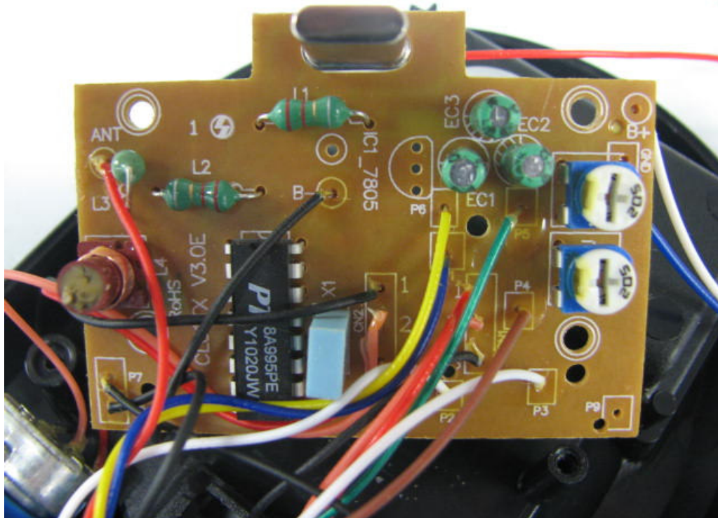
Transmitter (Internal view)
