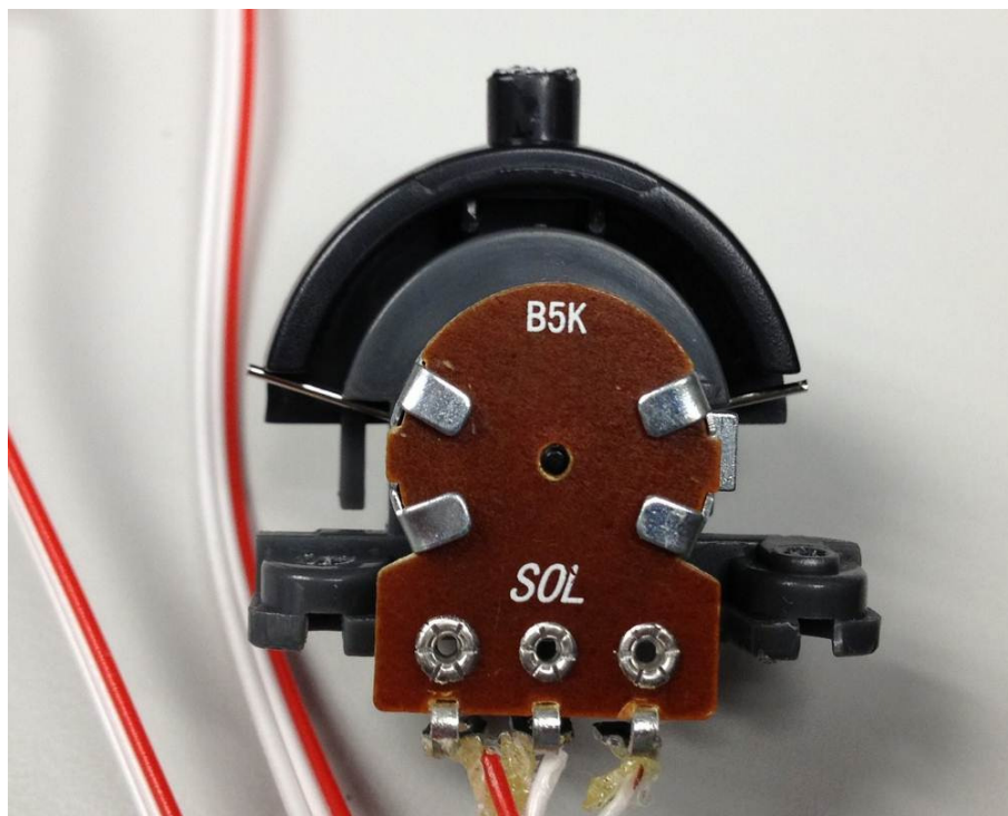
Internal View
