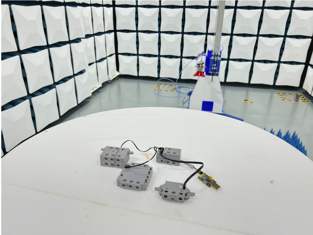
Set up for Radiated Emission Above 1G
