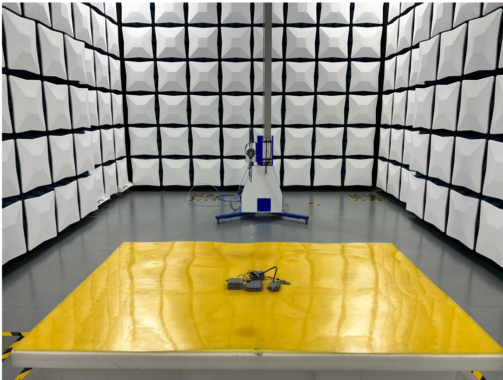
Set up for Radiated Emission Below 200M~1G
