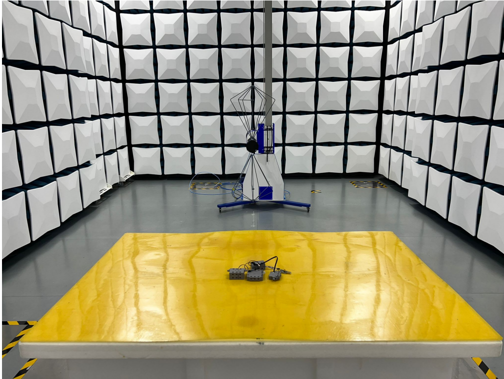
Set up for Radiated Emission 30M~200MHz
