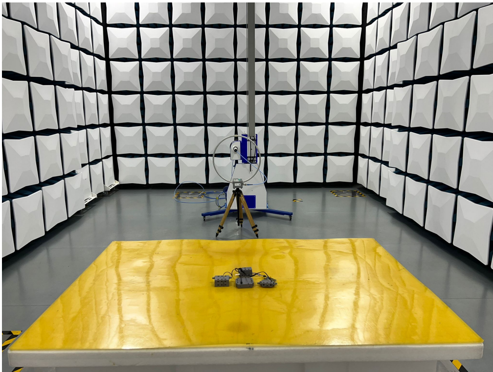
Set up for Radiated Emission Below 30MHz
