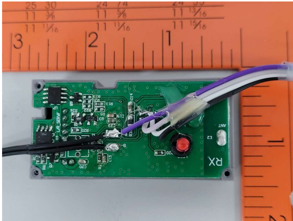
Internal View – Radio
