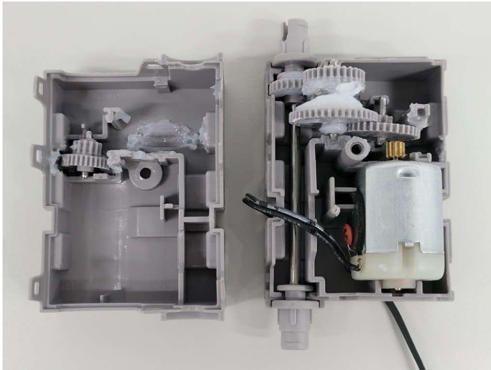
Internal View – Gear Box
