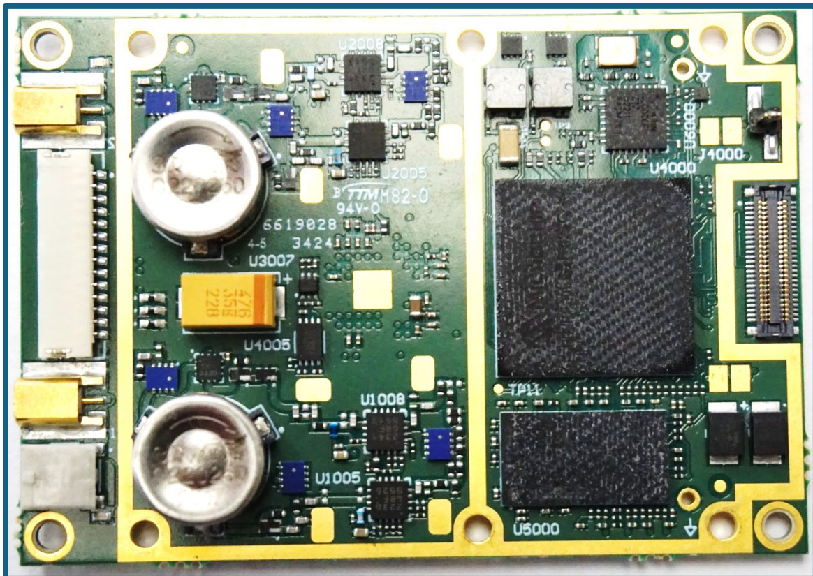
Digital side
