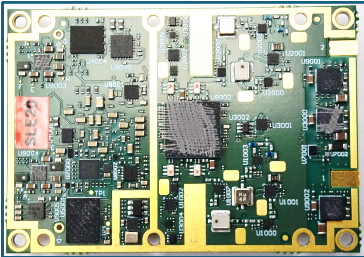
RF side
