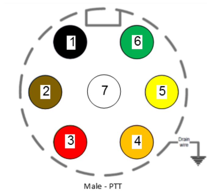
Figure 15 SC4200 PTT Pinout Diagram (Cable Side)
