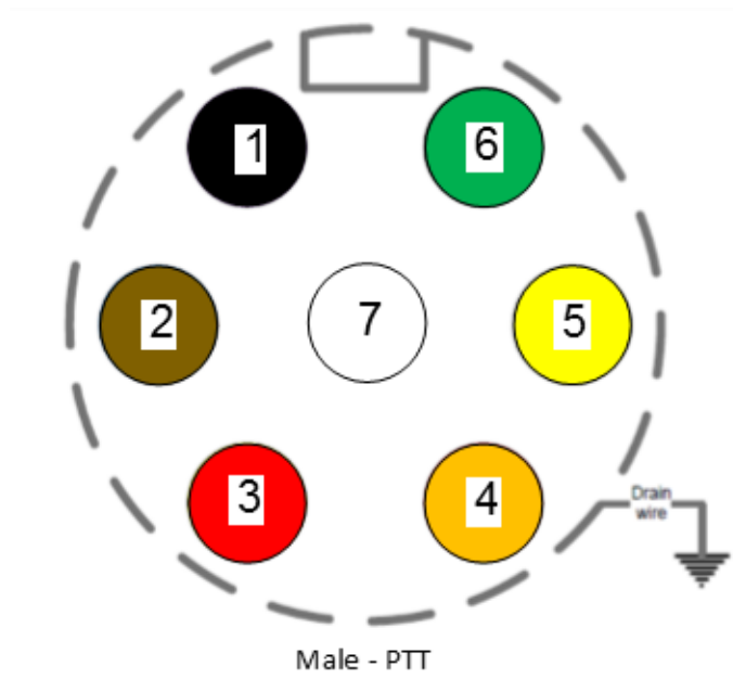
Figure 12 SC4400 PTT Pinout Diagram (Cable Side)
