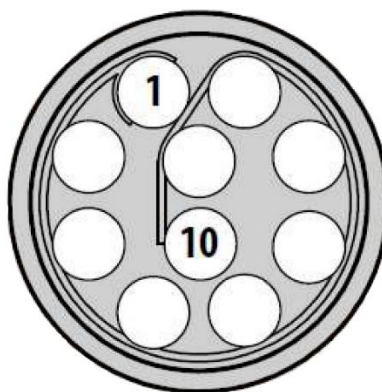
Figure 8 SC4200E Power (Optional)/Serial/Ethernet Pinout Diagram (Cable Side)
