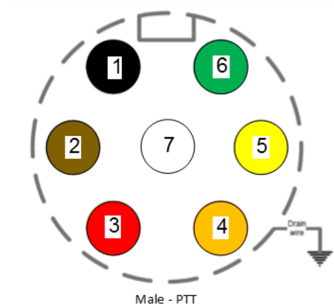
Figure 9 SC4200E PTT Pinout Diagram (Cable Side)
