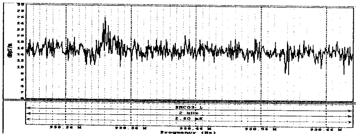
Fig.8. Fourth harmonic emission of unit 1. The maximum was found at 1.0-m height of the vertically polarized antenna.
