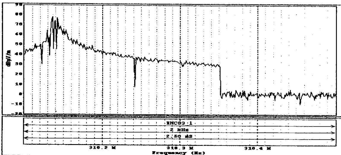
Fig.4. Emission from unit 1 command module. The DSI 2020 receiver uses peak detection for its sweeps. The antenna was horizontally polarized and 1.0-m above the ground plane. The precipitous drop at 310.35 MHz resulted from the module turning off.
