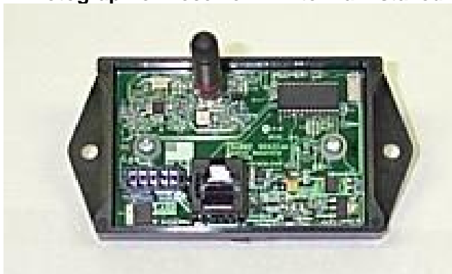
Photograph of Receiver – Antenna Installed
