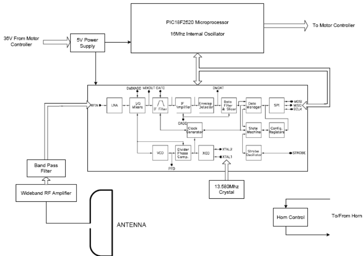
CS1882 DANE QuickKART Receiver Block Diagram
