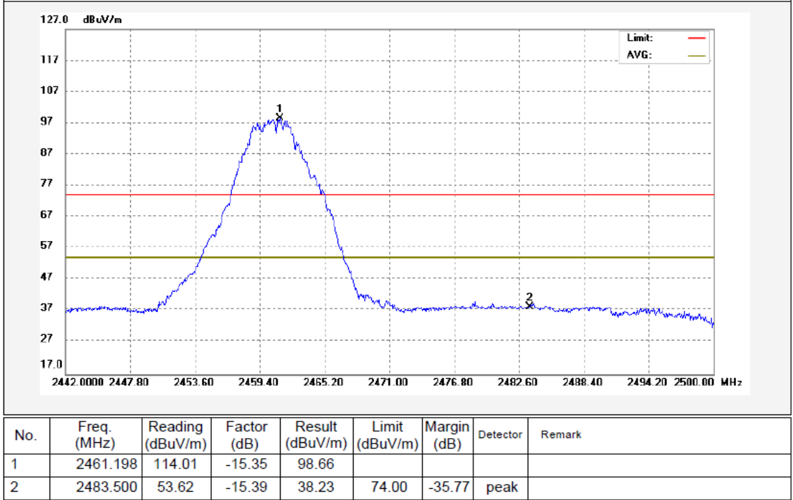
TX 11b: Band edge-right side Vertical
