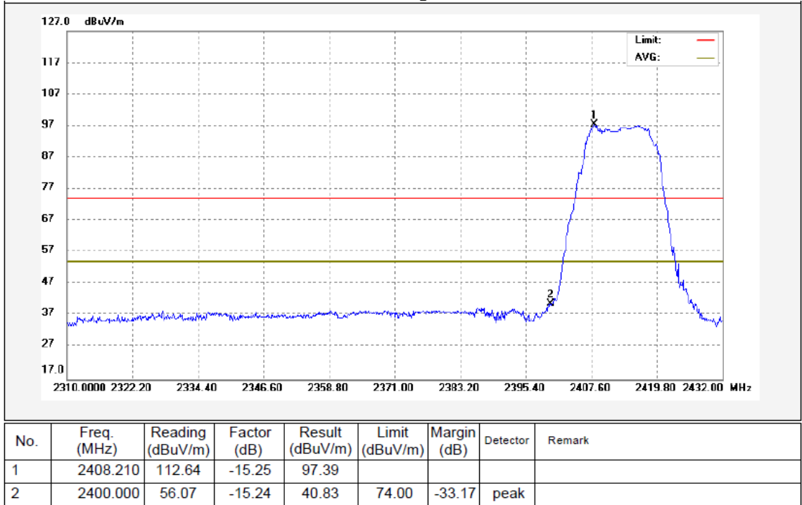
TX 11n HT20: Band edge-left side Vertical
