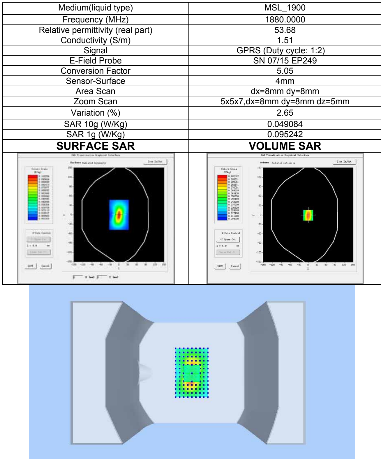
Plot 6: GPRS1900, Middle channel (Hotspot, Bottom side) Product Description: 3G Smart Phone Test Date: Jun 14,2017
