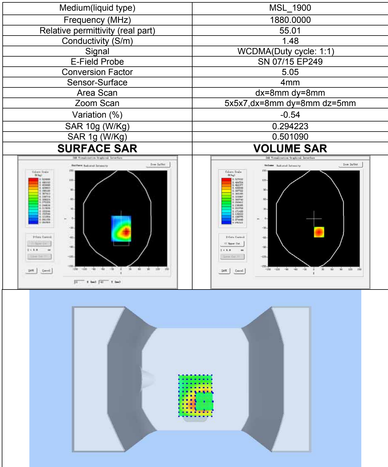
Plot 10: WCDMA BAND , Middle channel (Body-worn, Back Surface) Product Description: 3G Smart Phone Test Date: Jun 12,2017
