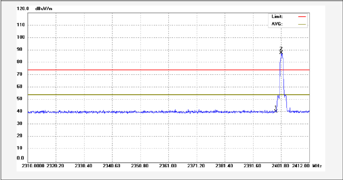
Pi/4 DQPSK Transmitting Band edge-left side Horizontal
