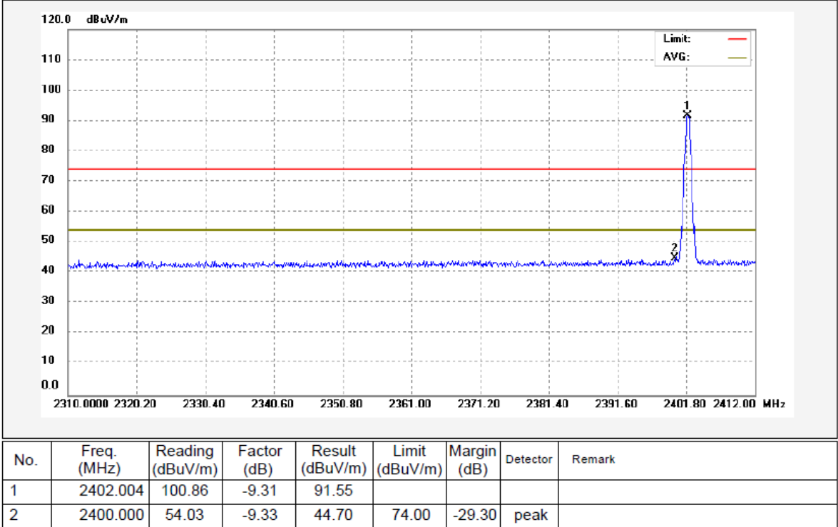
GFSK Transmitting Band edge-left side Vertical
