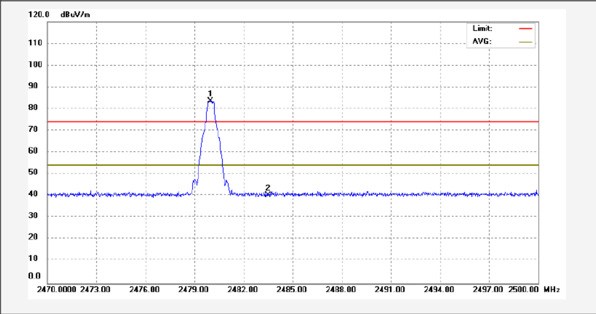
GFSK Transmitting Band edge-right side Vertical
