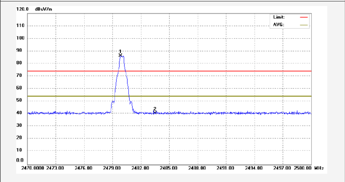
GFSK Transmitting Band edge-right side Horizontal
