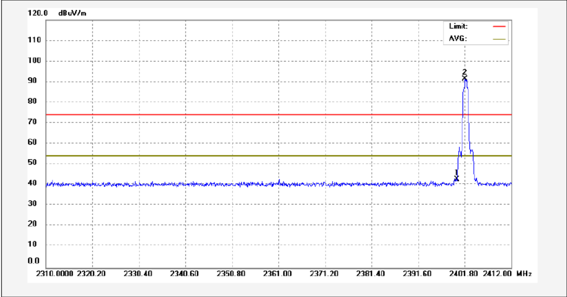
Pi/4 DQPSK Transmitting Band edge-left side Vertical
