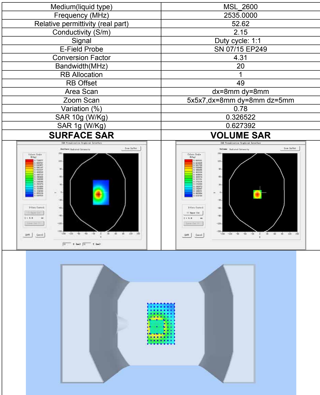
Plot 16:LTE BAND7, Middle channel (Data mode, Bottom edge) Product Description:Mobile Phone Test Date: Apr. 05, 2017
