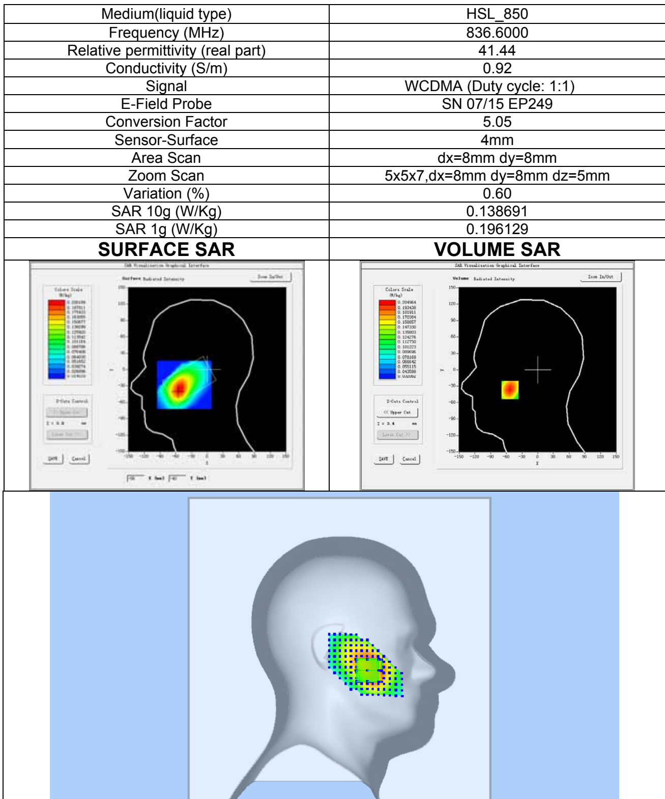
Plot 7: WCDMA BAND V, Middle channel (Left Head Cheek) Product Description: Mobile Phone Test Date: Apr. 06, 2017
