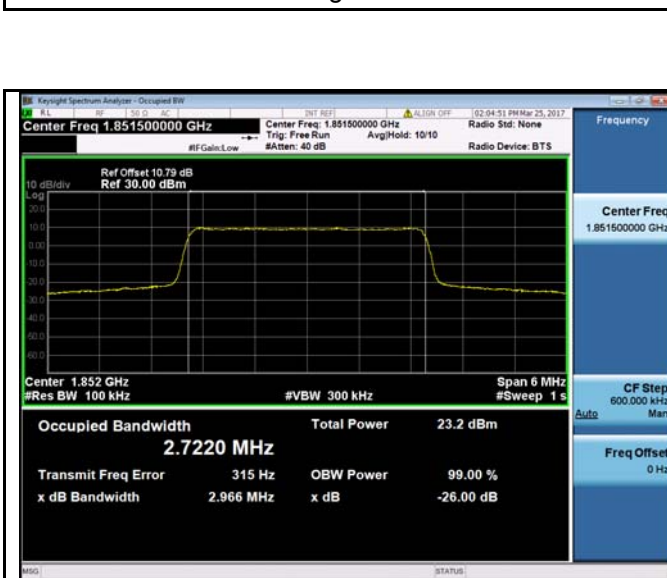
LTE band 2 - Low CH QPSK-3
