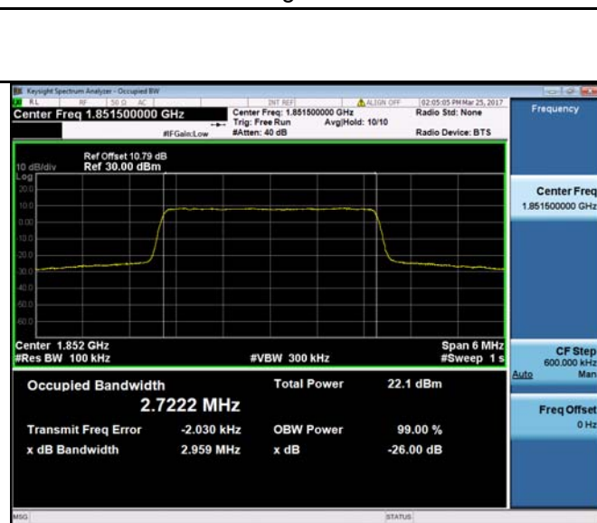
LTE band 2 - Low CH 16QAM-3
