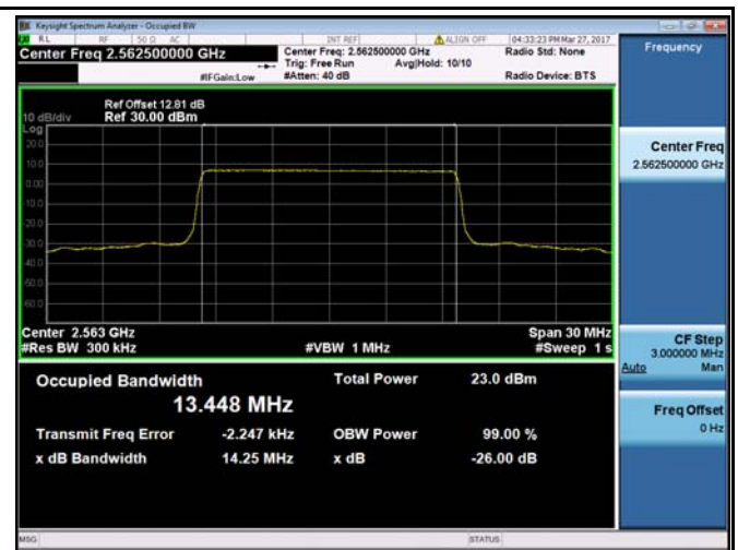
LTE band 7 - High CH 16QAM-15
