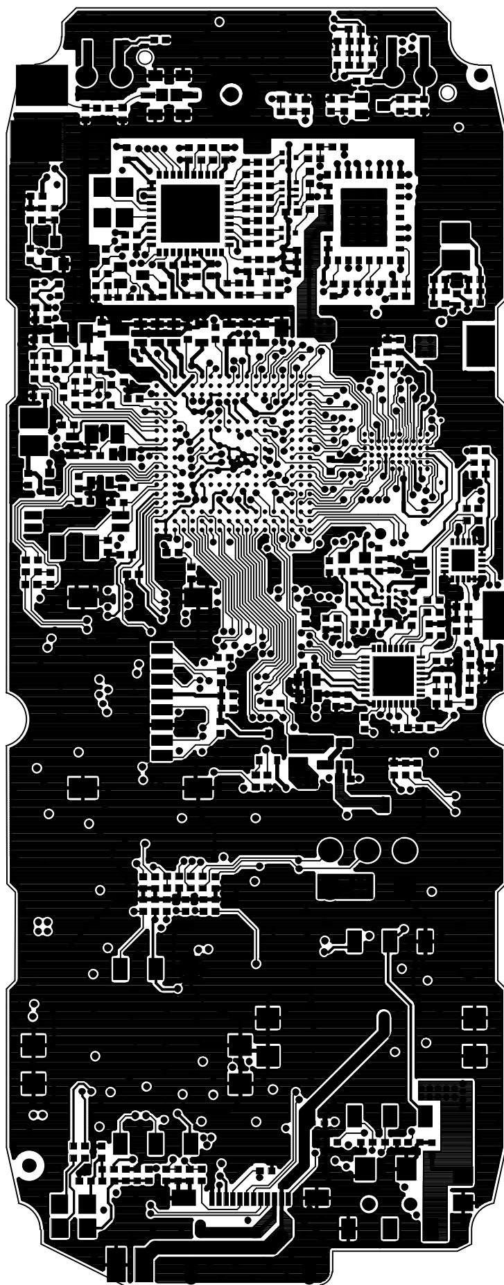
Top routing
