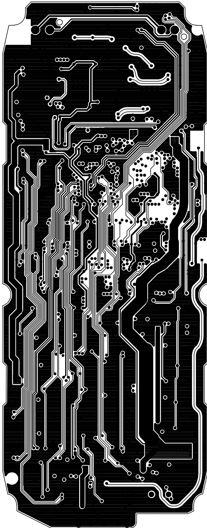
Layer3 routing
