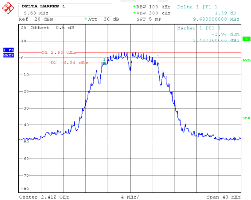
802.11b Low Channel
