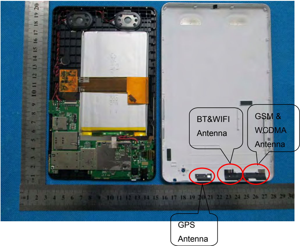
OPEN VIEW OF EUT-1
