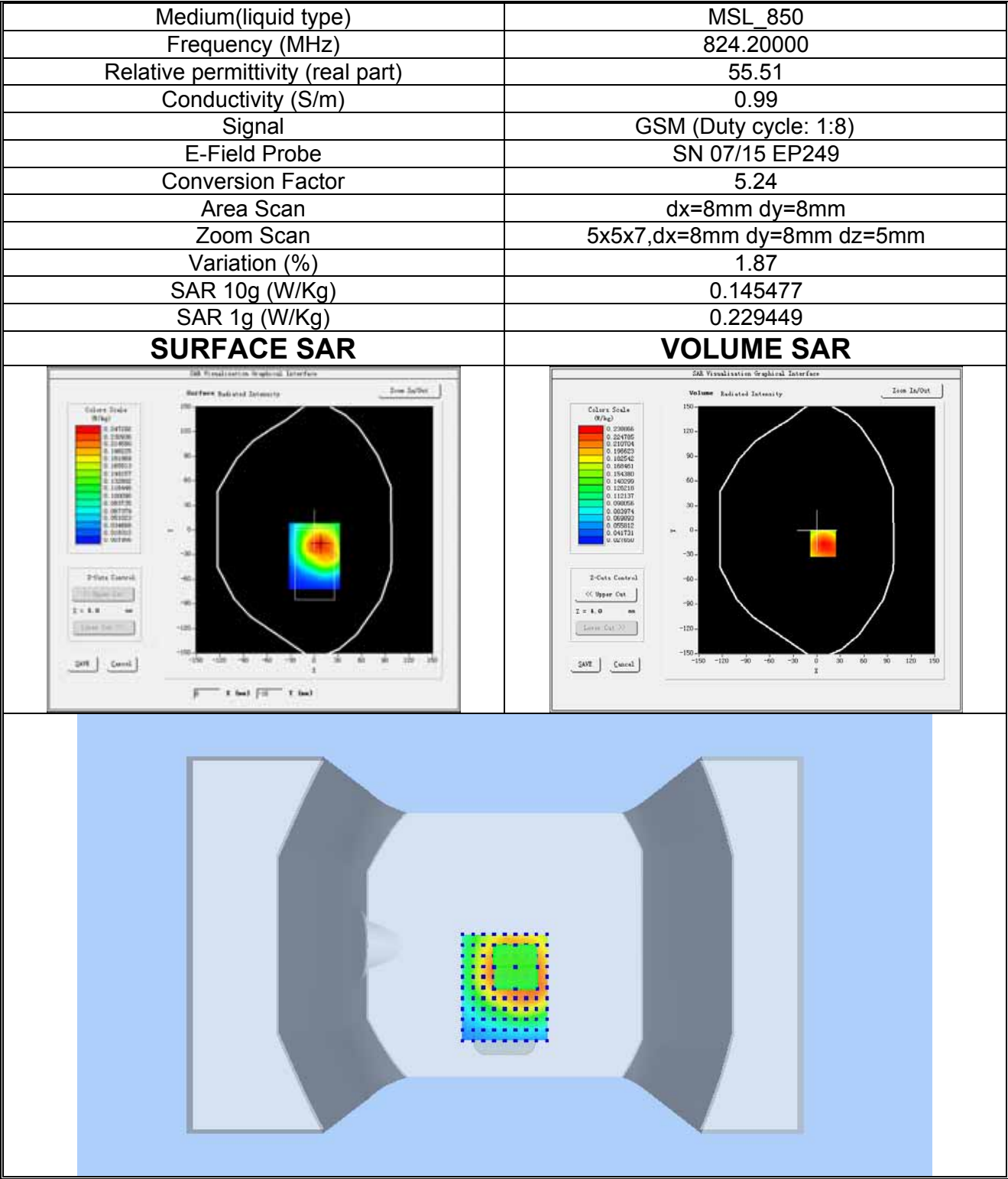
Plot 2: GSM850MHz, Low channel (Body-worn, Front Surface) Product Description:Mobile Phone Test Date: 2018-05-22
