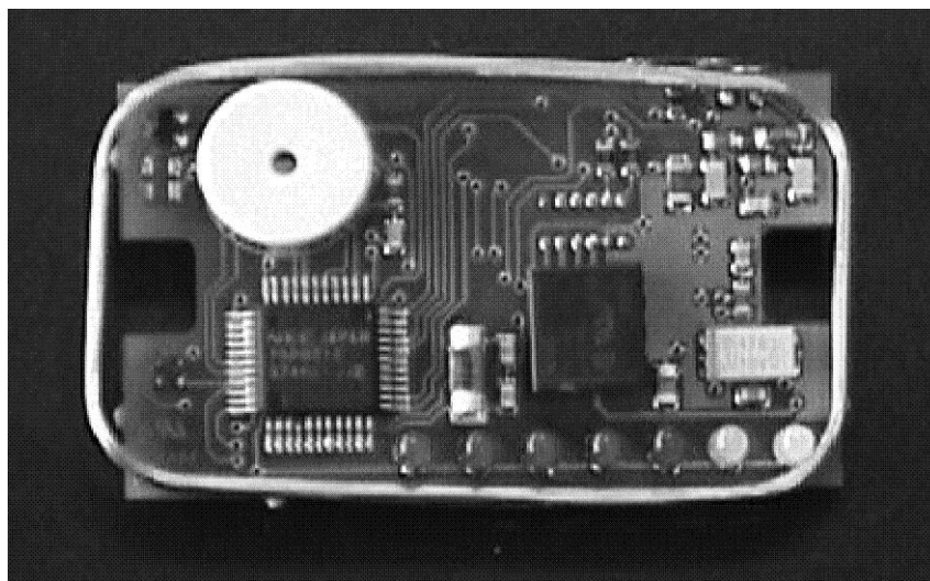
Figure 2 - PCB Side 2
