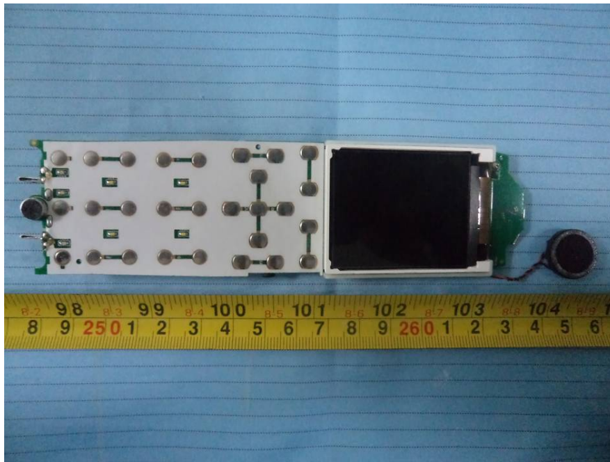
EUT – Main Board Bottom with LCD Front View
