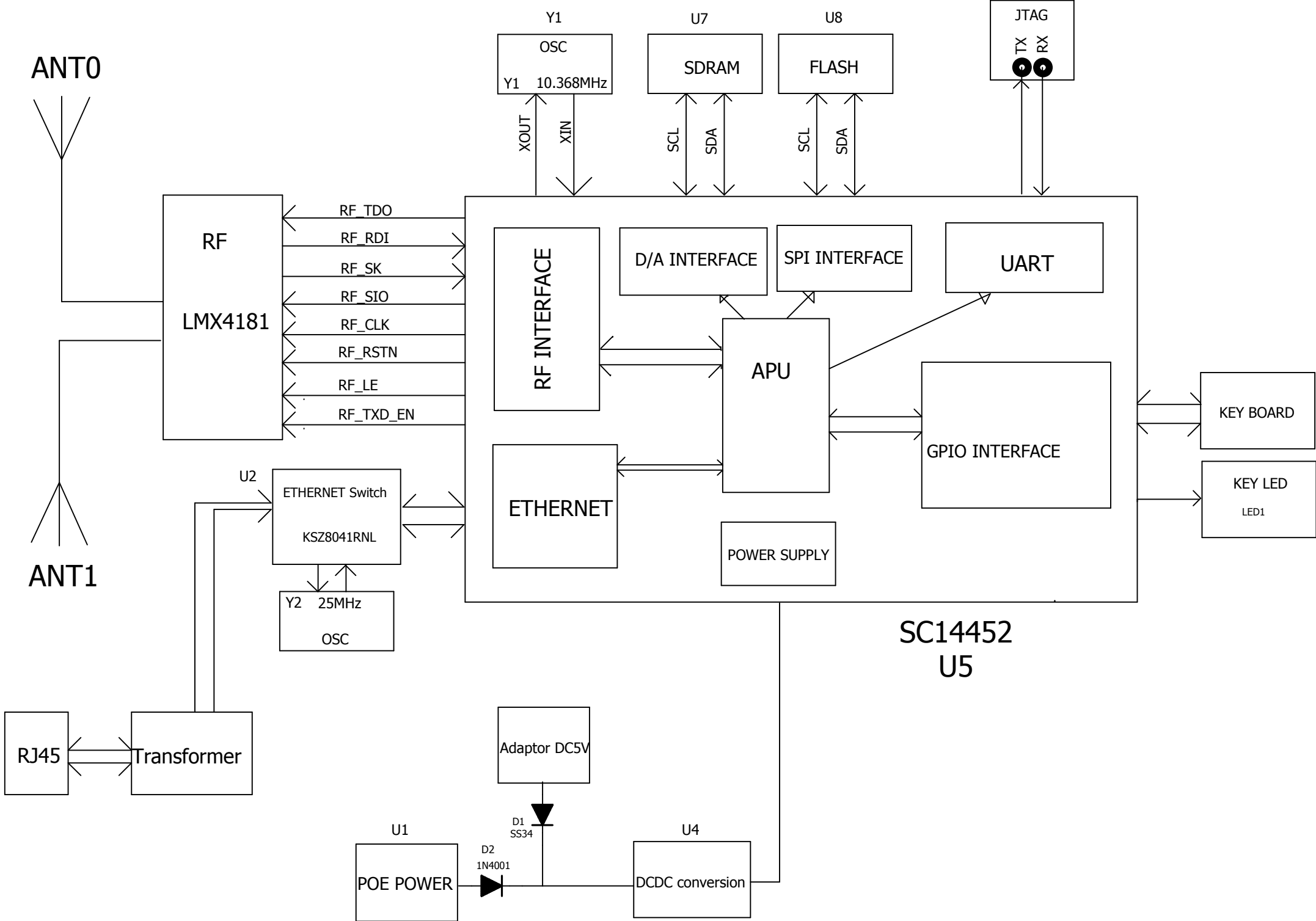
IP160S_BASE_BLOCK DIAGRAM
