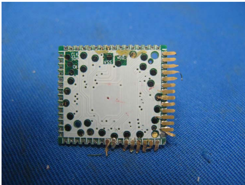
Base Unit (GPCEO48/63) PCB solder side
