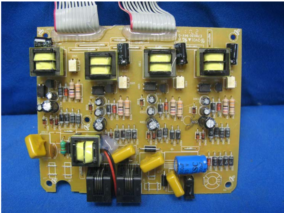
Base Unit Power Board front side
