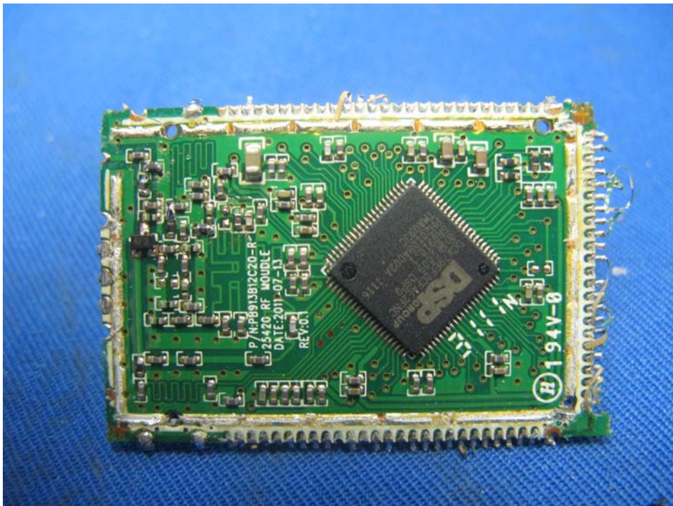
Base Unit DECT RF PCB comp side
