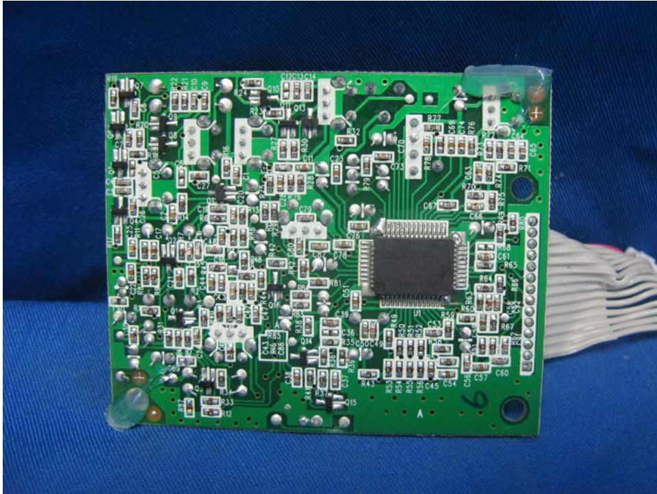
Base Unit another Main PCB solder side
