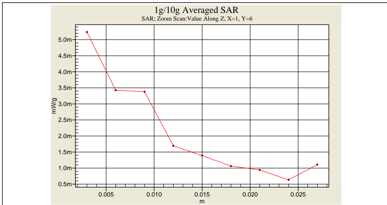
Body SAR Measurement _ CH2 _ Back to Phantom 2mm separation
