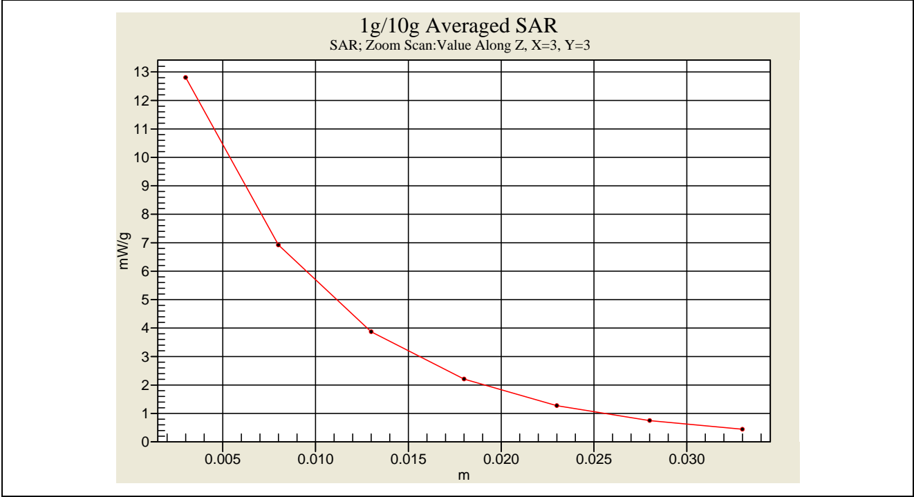
Head-Tissue-Simulating-Liquid 1900MHz
