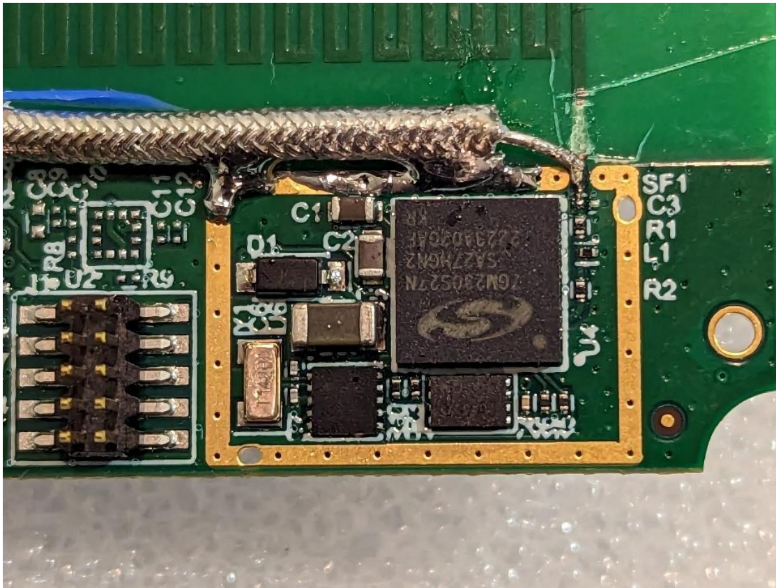
Photograph 3 – View of Circuitry Under the Shield
