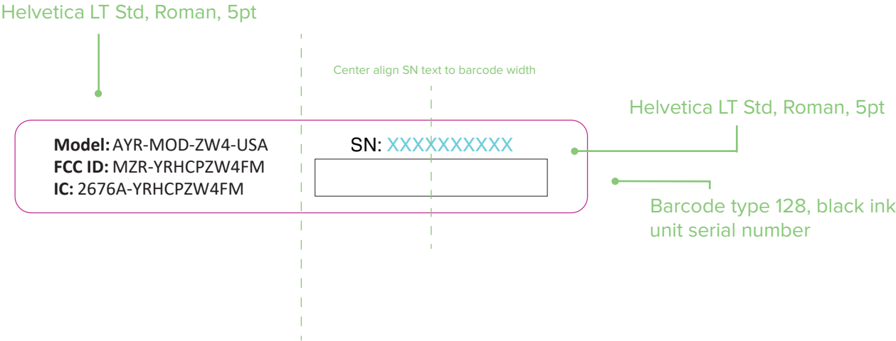
ARTWORK LAYOUT, SCALE 2:1
