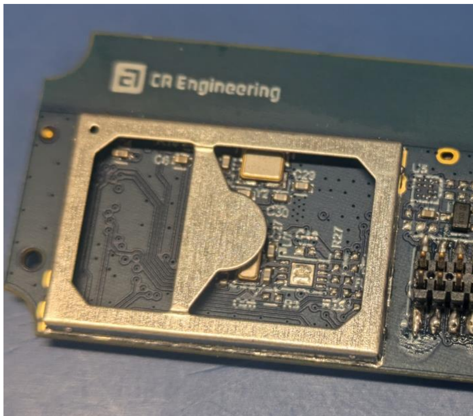
Photograph 3 – View of Circuitry Under the Shield
