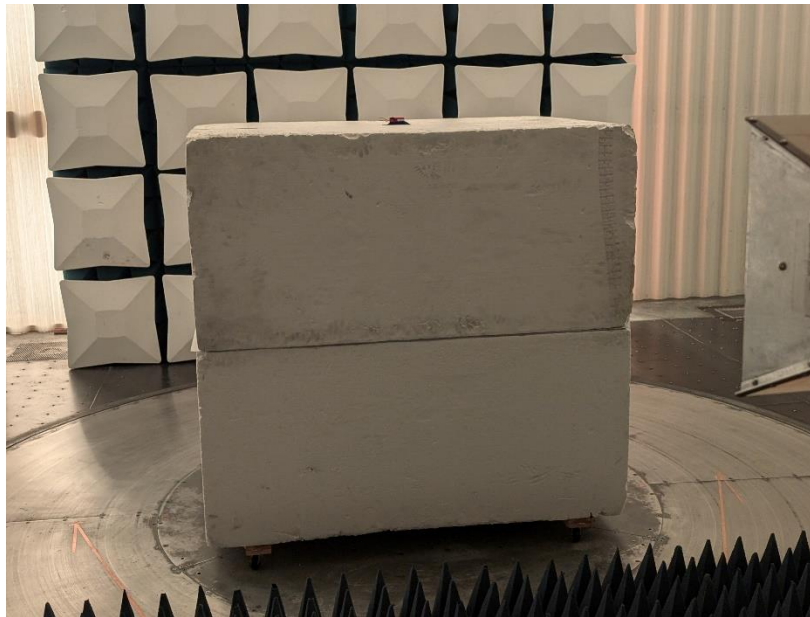
Photograph 13: Back View Radiated Emissions Configuration (“Long Edge” Orientation) – Frequencies Above 1000 MHz
