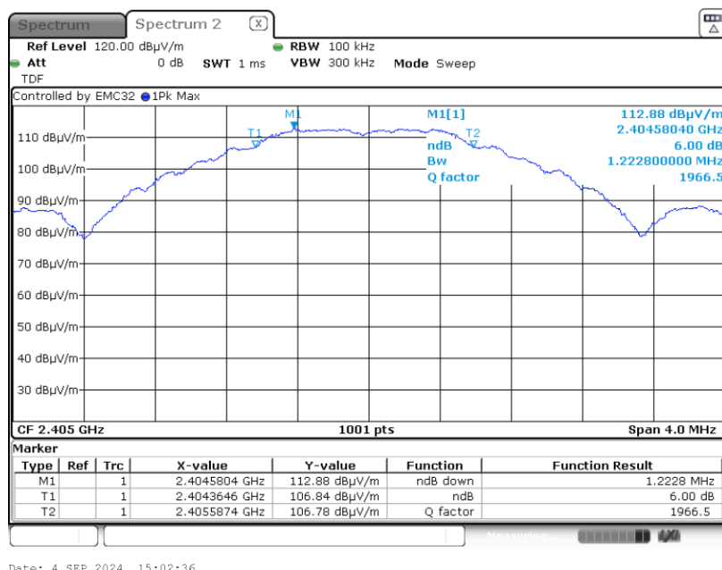
Graph 1: Lowest Channel Bandwidth
