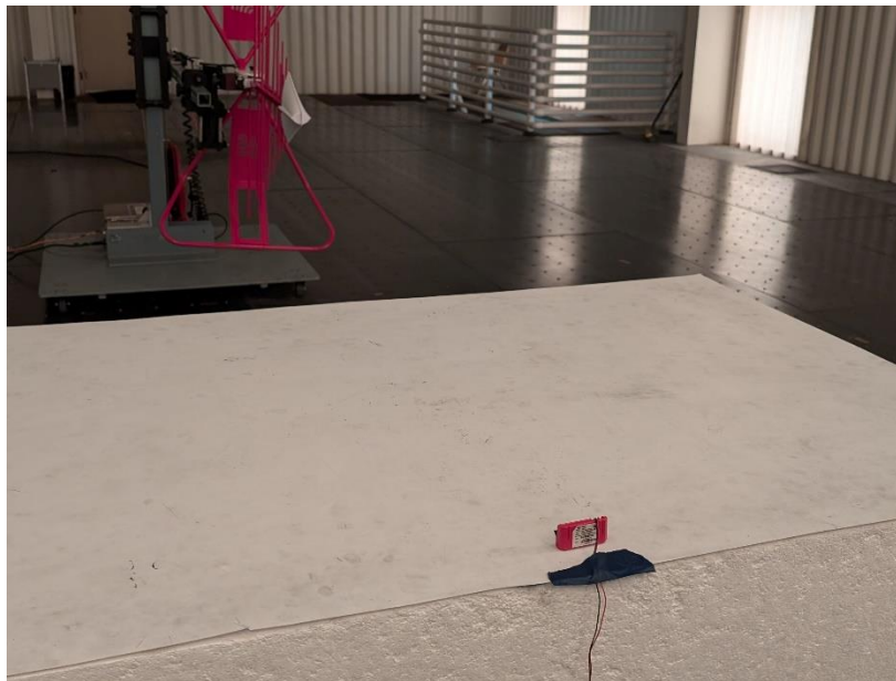
Photograph 6: Front View Radiated Emissions Configuration (‘Long Edge’ Orientation) – Frequencies Below 1000 MHz
