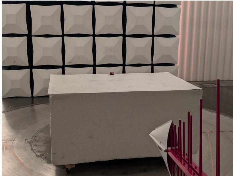
Photograph 7: Back View Radiated Emissions Configuration (‘Long Edge’ Orientation) – Frequencies Below 1000 MHz
