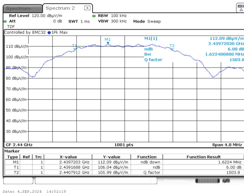
Graph 2: Middle Channel Bandwidth
