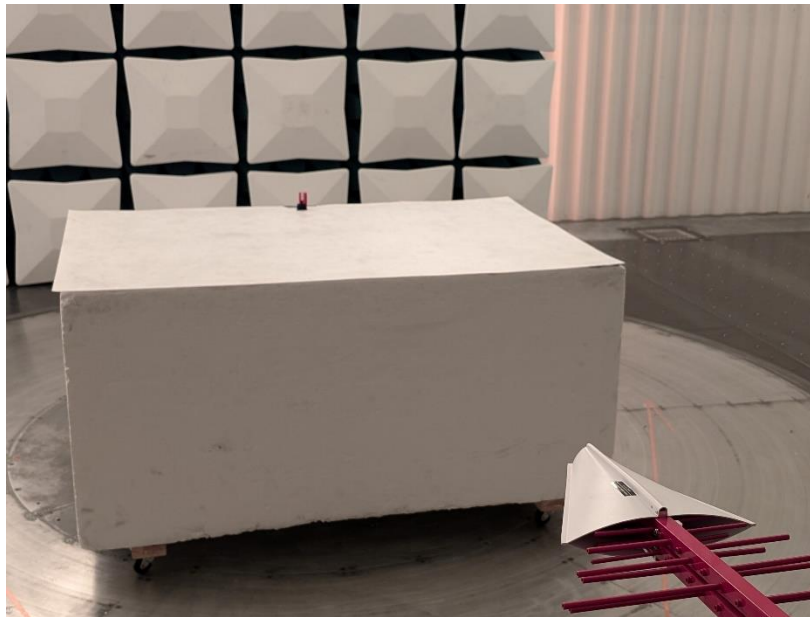
Photograph 9: Back View Radiated Emissions Configuration (‘Short Edge’ Orientation) – Frequencies Below 1000 MHz
