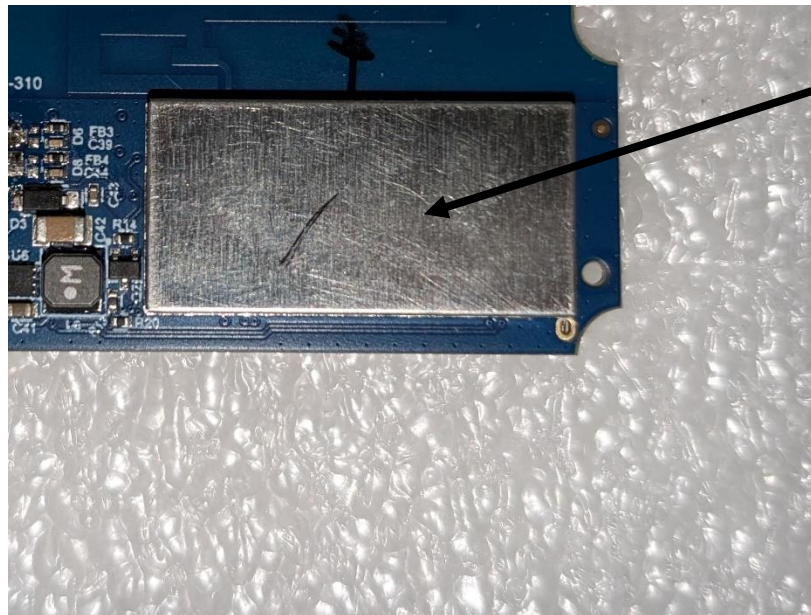
Photograph 26: Back View of the PCB
