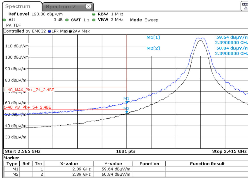
Graph 9: Radiated Lower Restricted Band Edge Plot (Radio Level 0dBm, Amp +20dB)
