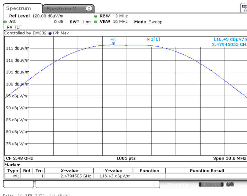
Graph 6: Highest Channel Output Power Plot
