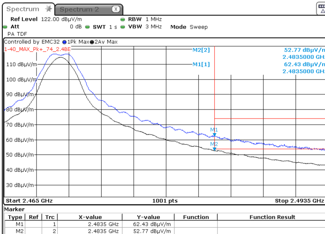
Graph 10: Radiated Upper Authorized and Restricted Band Edge Plot (Transmitting 2470MHz, Radio Level 0dBm, Amp +20dBm)
