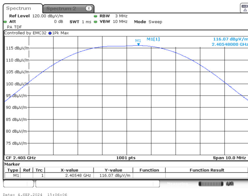
Graph 4: Lowest Channel Output Power Plot
