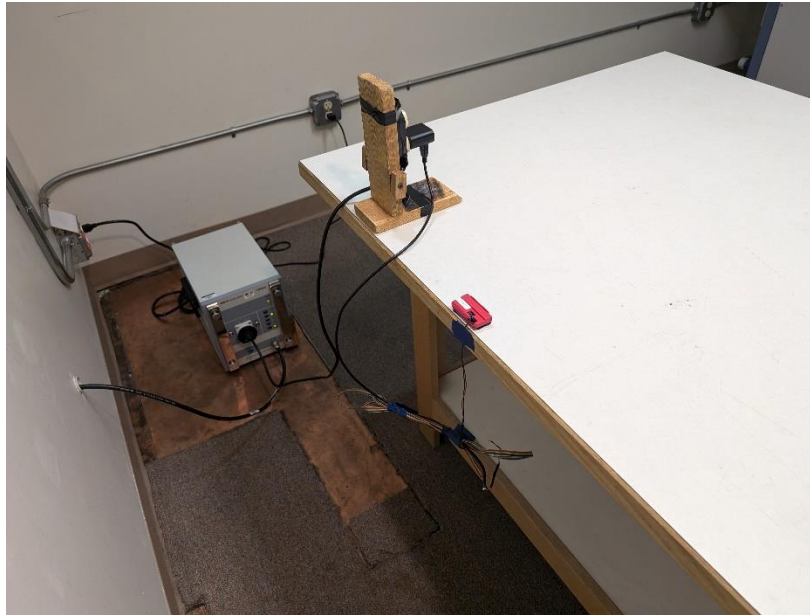
Photograph 17: Back View Conducted Emissions Worst-Case Configuration
