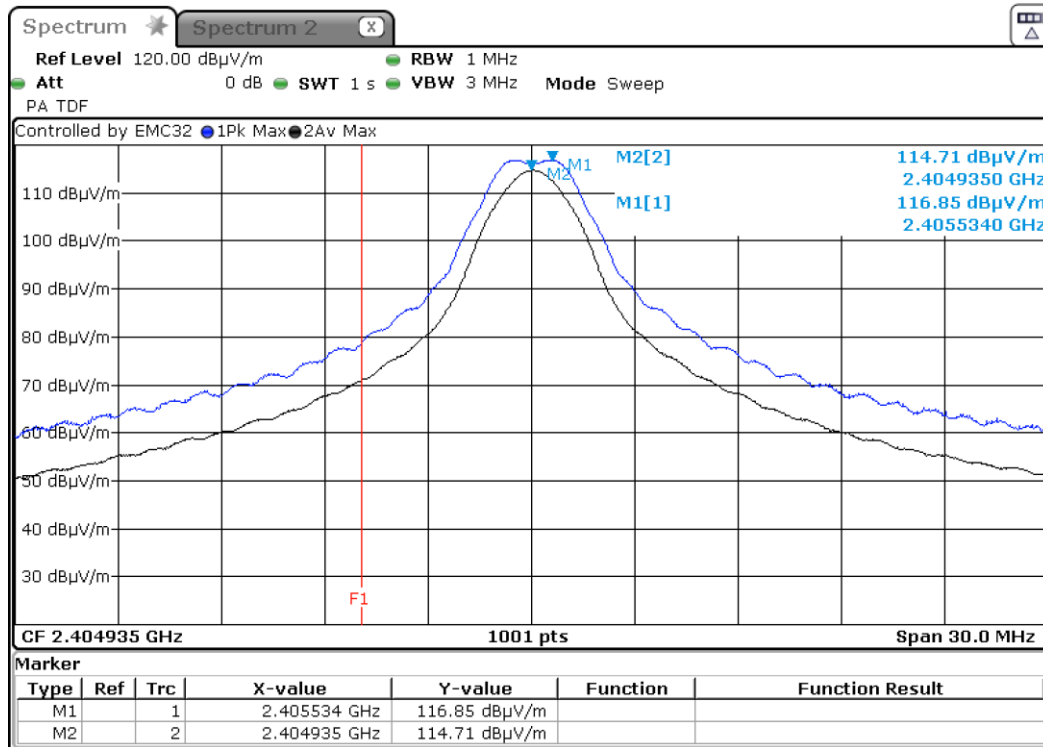
Graph 7: Radiated Lower Authorized Band Edge Plot (In-Band Measurement, Radio Level 0dBm, Amp +20dB)
