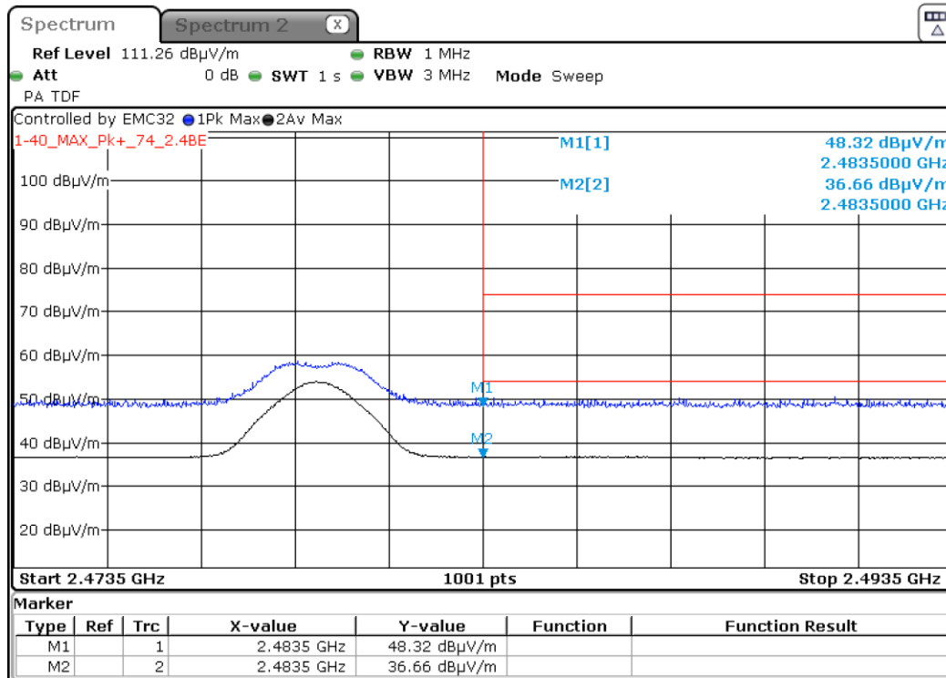
Graph 12: Radiated Upper Authorized and Restricted Band Edge Plot (Transmitting 2480MHz, Radio Level -23dBm, Amp +0dBm)
