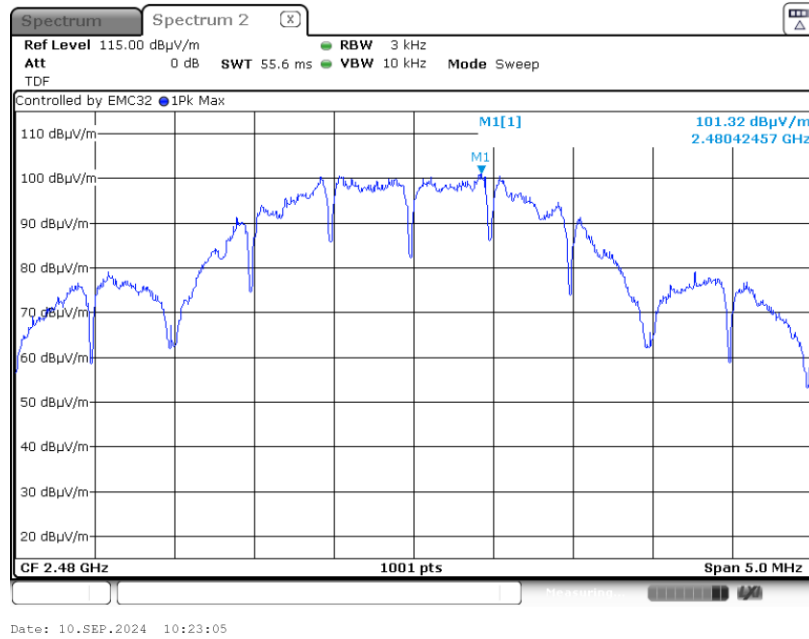
Graph 15: Highest Channel Output 3 kHz PSD Plot
