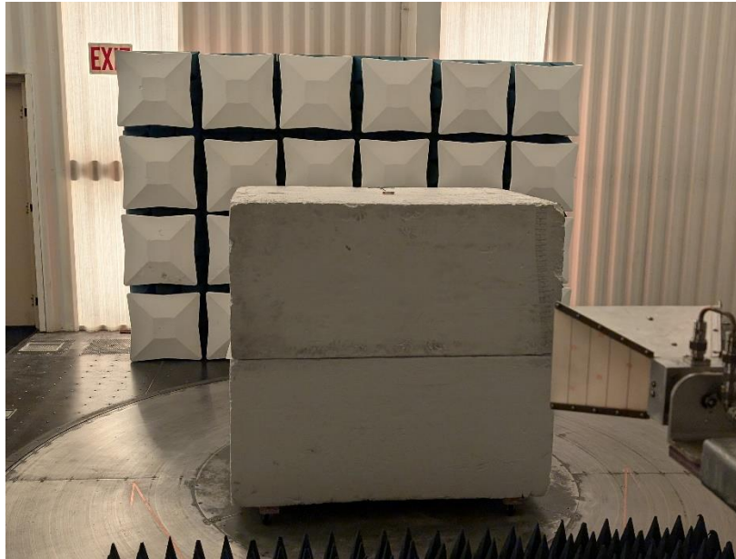
Photograph 11: Back View Radiated Emissions Worst-Case Configuration (“Laying Flat” Orientation) – Frequencies Above 1000 MHz
