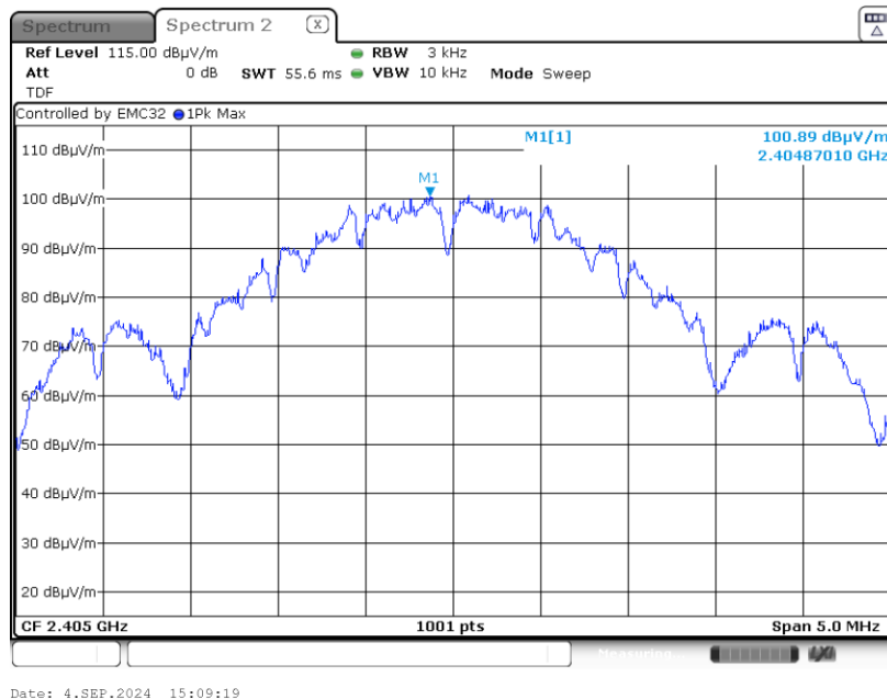
Graph 13: Lowest Channel 3 kHz PSD Plot
