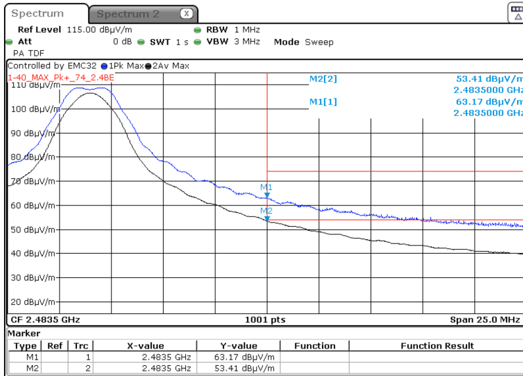
Graph 11: Radiated Upper Authorized and Restricted Band Edge Plot (Transmitting 2475MHz, Radio Level -14dBm, Amp +20dBm)
