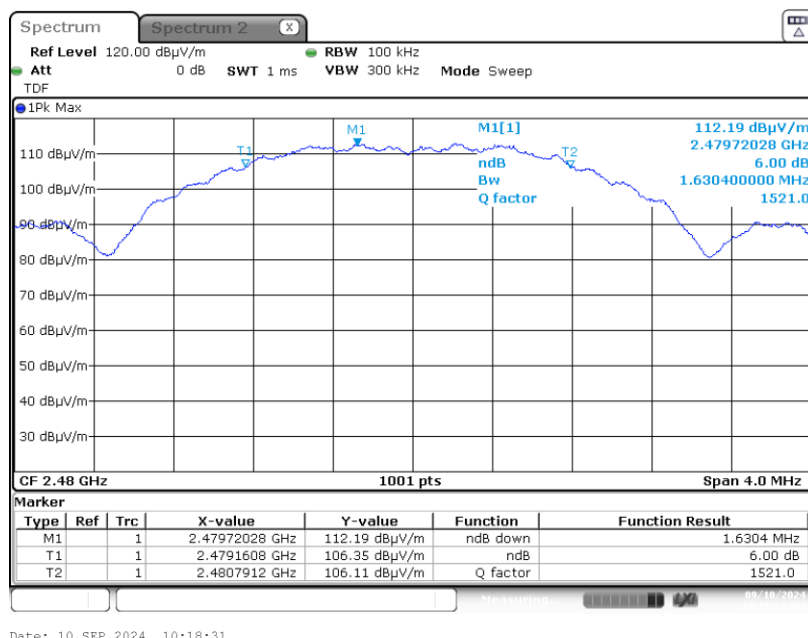
Graph 3: Highest Channel Bandwidth
