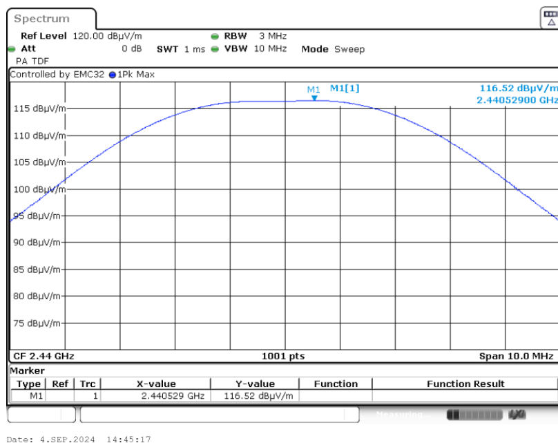
Graph 5: Middle Channel Output Power
