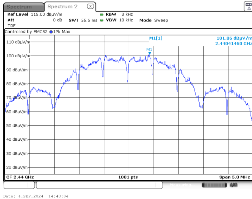
Graph 14: Middle Channel 3 kHz PSD Plot
