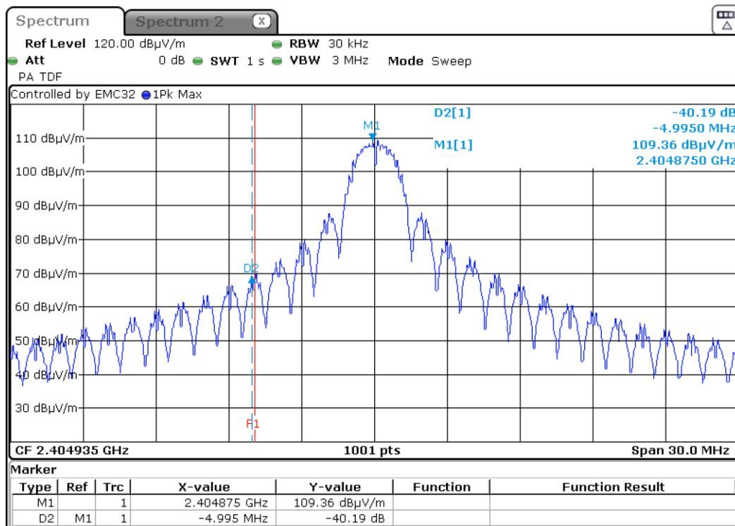
Graph 8: Radiated Lower Authorized Band Edge Plot (Delta Measurement, Radio Level 0dBm, Amp +20dB)
