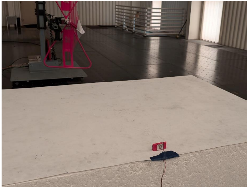
Photograph 2: Back View Radiated Emissions Worst Case below 1000 MHz Configuration
