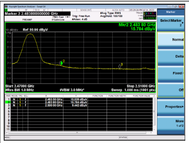
Channel 25 band edge (Average)
