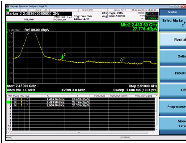
Channel 25 band edge (Peak)
