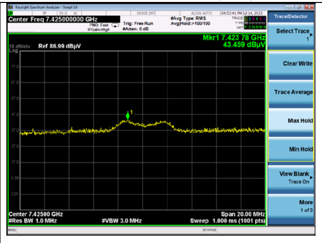
Channel 25 3 rd Harmonic (Peak)
