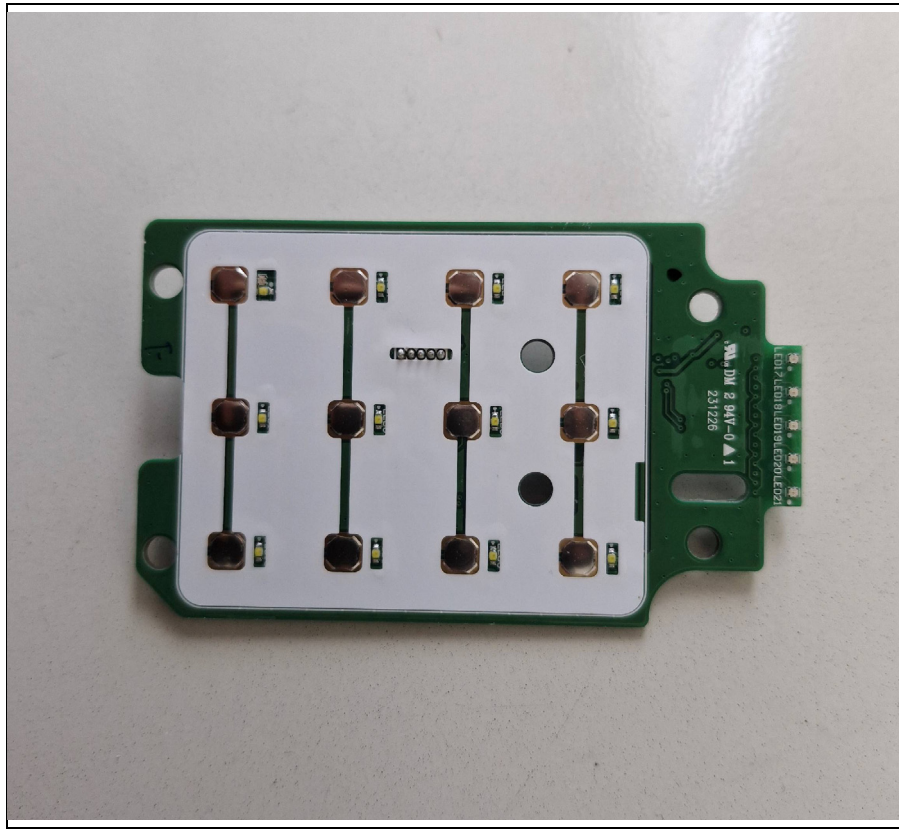
Bottom view of Sub PCB1
