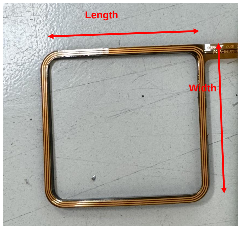
FCPB Antenna(YMB614)
