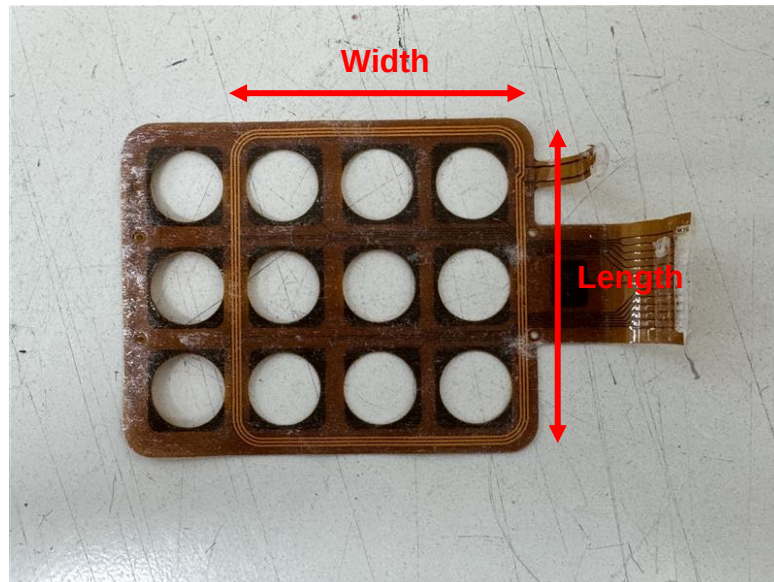
FCPB Antenna(YMB614)
