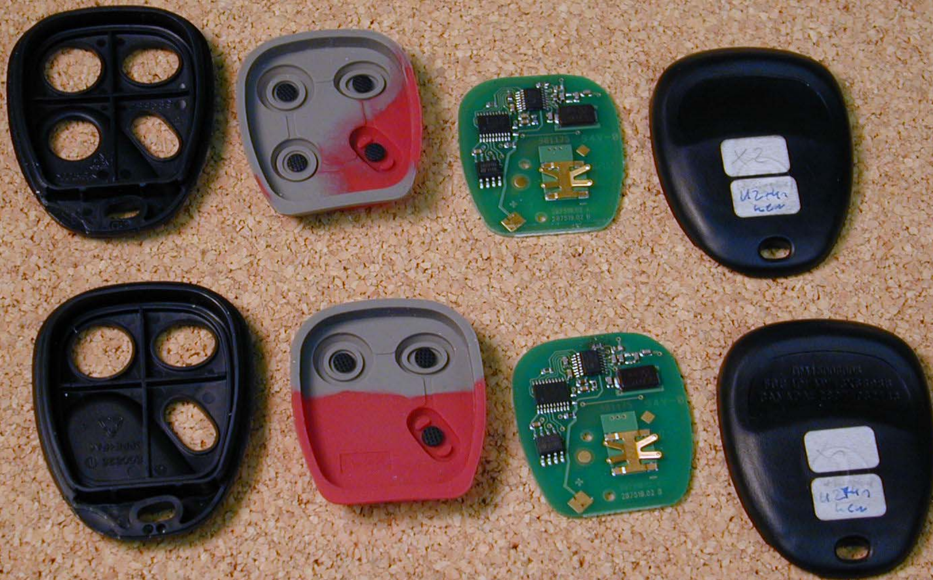
DUT Case Open (bottom) 3 Button and 4 Button Parts
