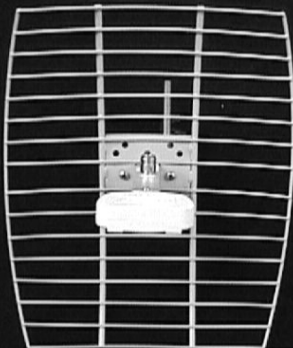
HYPERLINK HG2415G GRID ANTENNA
