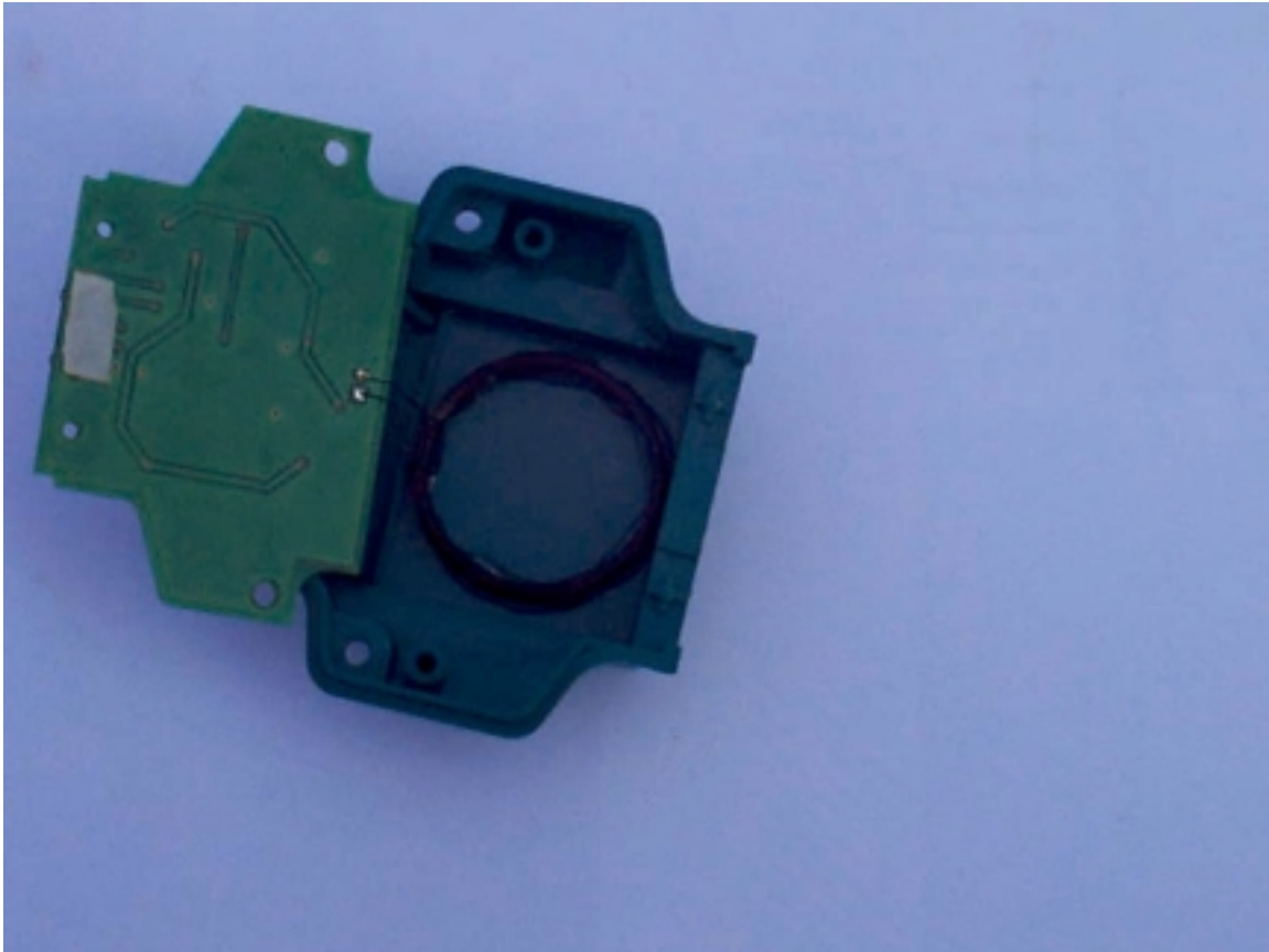
Figure 3 Coupling Coil
