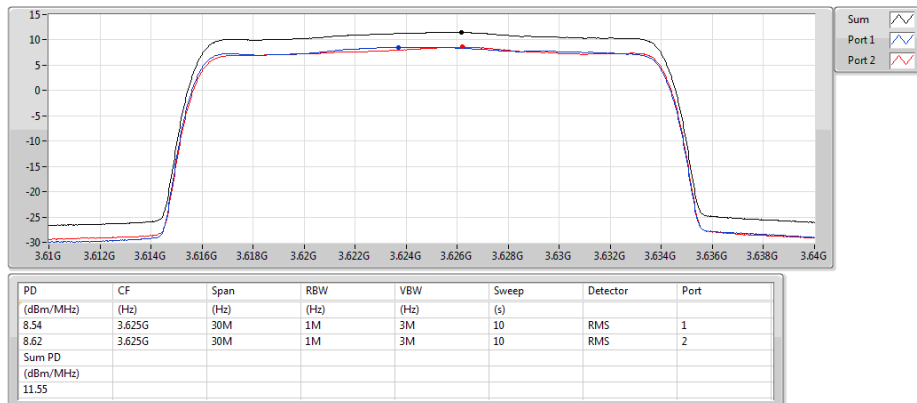
Band 48_LTE_20MHz_Nss1,16QAM_2TX 3625MHz_16QAM_RB 100,#RB 0
