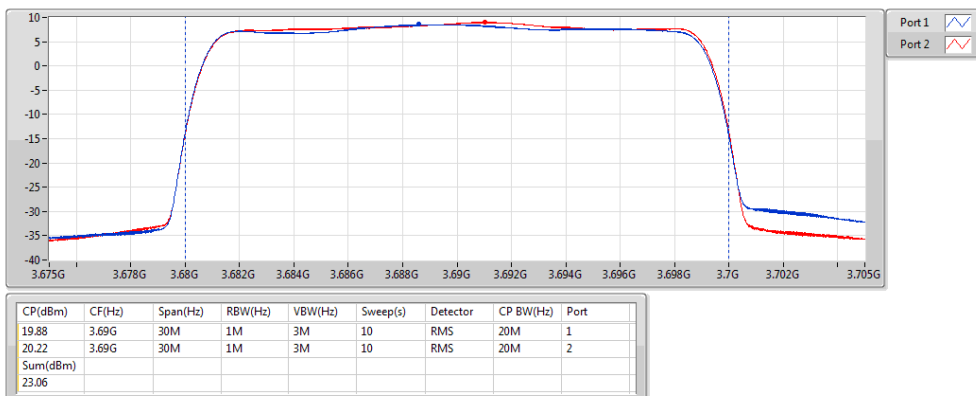
Band 48_LTE_20MHz_Nss1,16QAM_2TX 3690MHz_16QAM_RB 100,#RB 0
