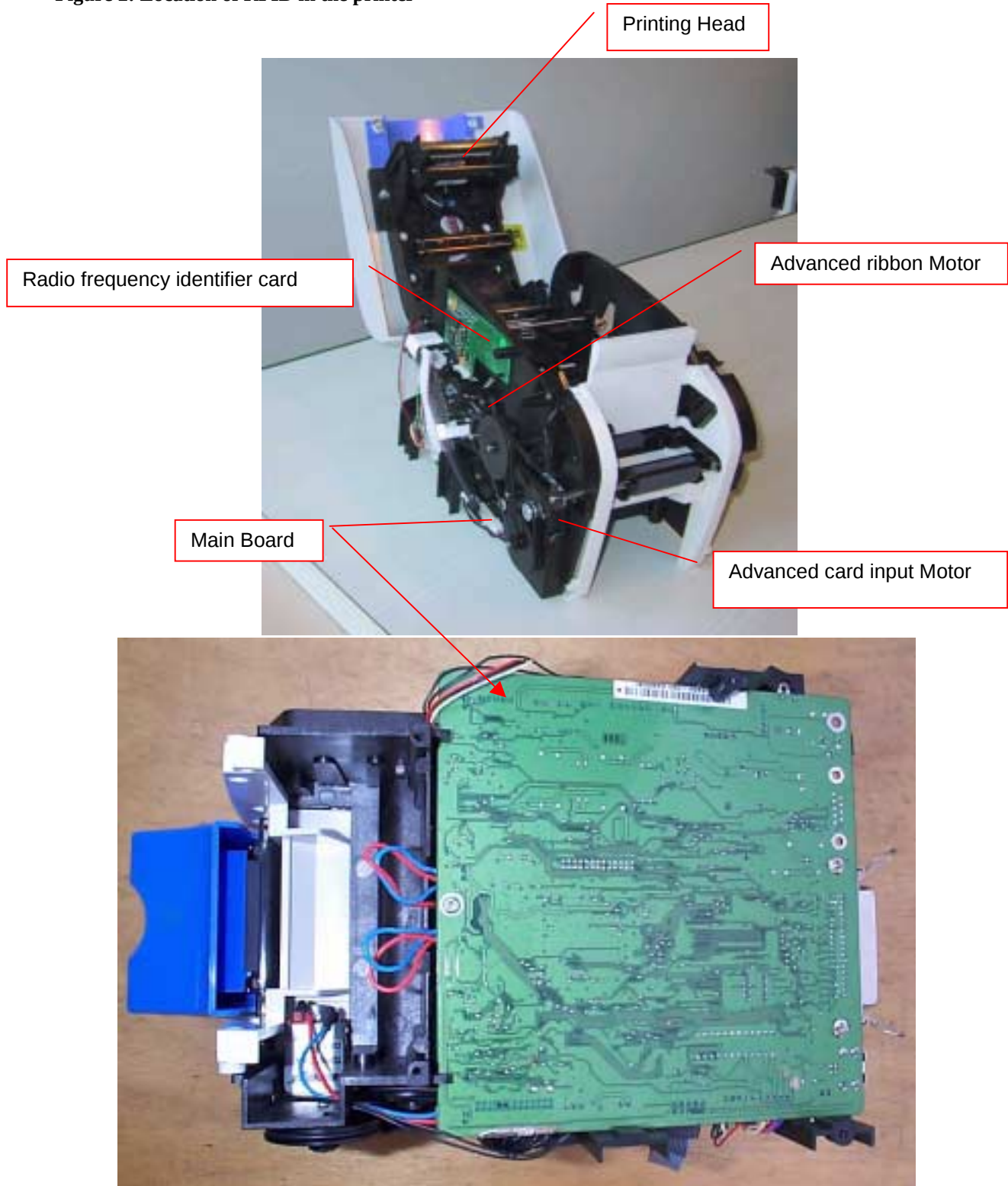
Figure 2: Location of RFID in the printer
