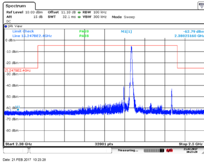
Figure 8.3.1: Bandedge Measurement
