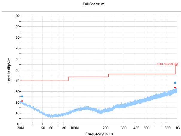
Figure 8.3.3: Radiated spurious emissions, 30-1000MHz
