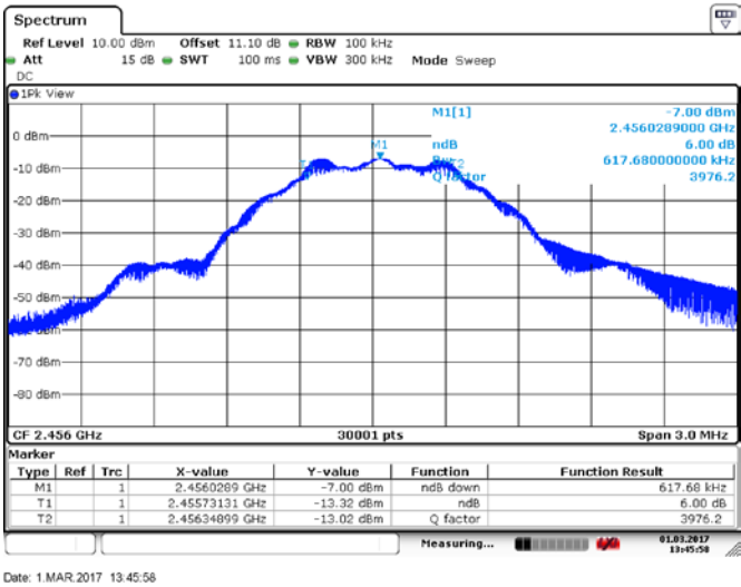
Figure 8.1-1: 6 dB bandwidth
