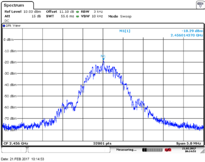
Figure 8.4-1: PSD
