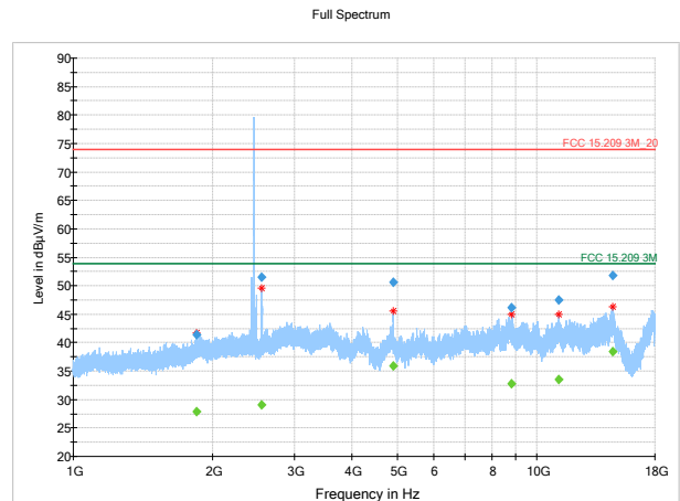
Figure 8.3.4: Radiated spurious emissions, 1-18GHz
