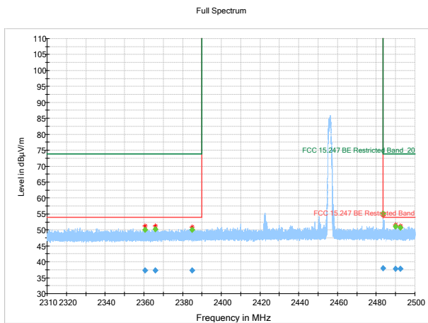
Figure 8.3.5: Radiated Bandedge in Restricted Band
