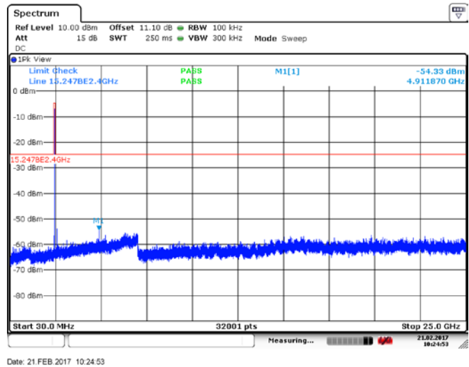
Figure 8.3.2: Conducted spurious emissions
