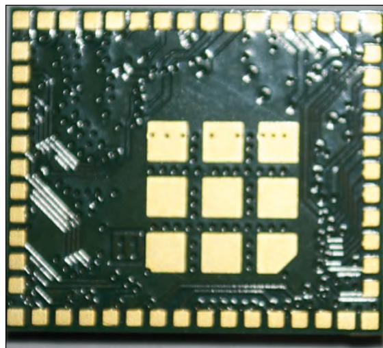
Figure 2: Bottom View
