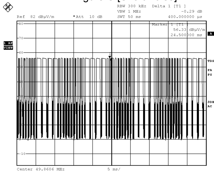
Figure C [Short Pulse]
