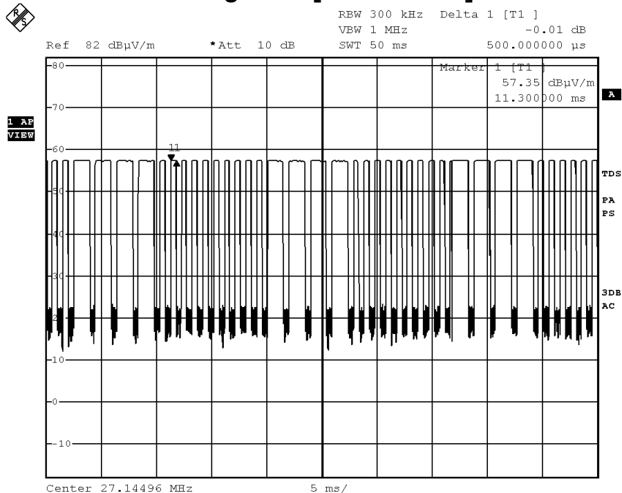
Figure C [Short Pulse]
