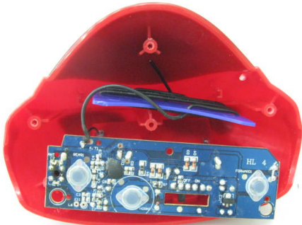
Front View of the product (Internal)
