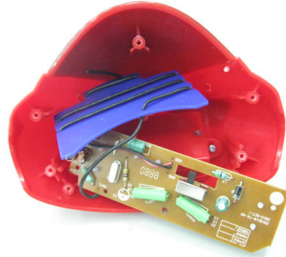
Rear View of the product (Internal)
